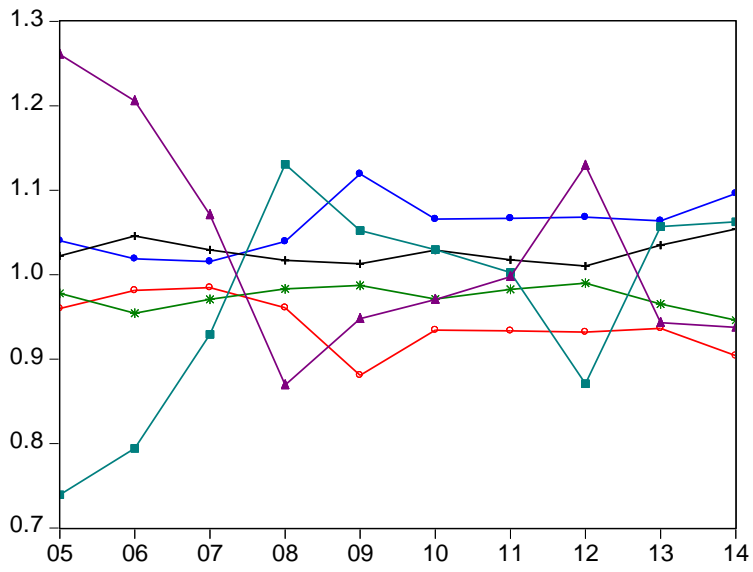
Figure 3 Transition paths for inefficiency scores for individual inputs x1, x2 and x3
