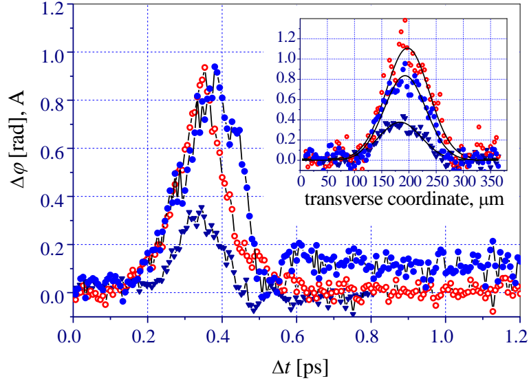
Figure 3. Time-resolved non-linear optical response of the glass samples: \text{As}_{40}\text{S}_{30}\text{Se}_{30} (filled triangles), \text{Ge}_{20}\text{Se}_{80} (open circles - \Delta\phi , filled circles - A ), E = 0.3 \mu\text{J} ; inset: transverse profiles of \Delta\phi and A at \Delta t = \Delta t^{max}
