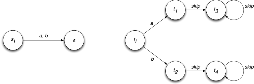
Figure 1: A transition system that does not satisfy (1) and (2) (left) and the corresponding system that satisfies (1) and (2) (right).
