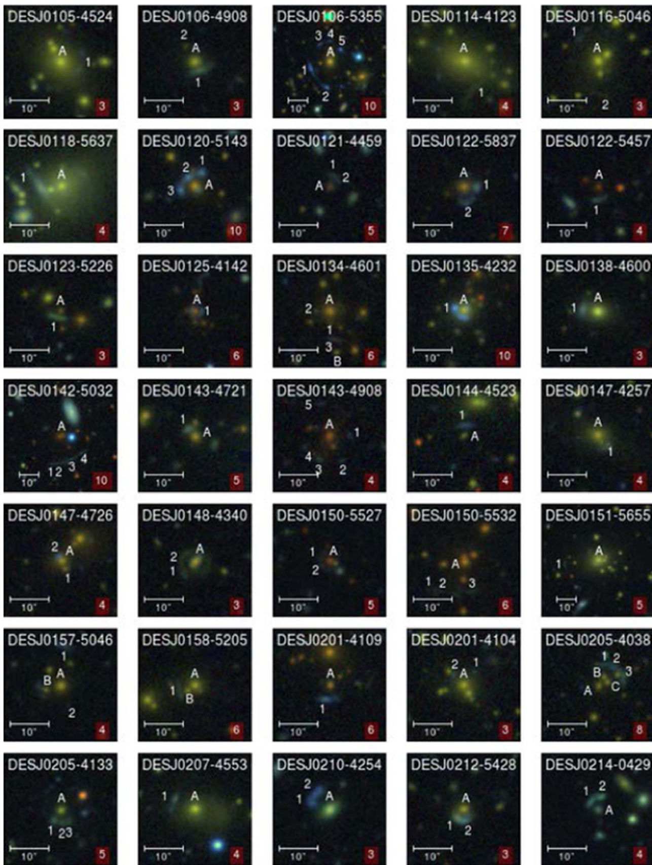
Figure 7. Second page of SL systems with ranks of 3 or more. Each cutout image has the visual inspection ranking displayed in a red box in the lower right hand corner. All images are oriented with north up and east left. Most of the cutouts are 30'' \times 30'' in size. Some of the largest systems are displayed with 60'' \times 60'' images, so that they fit well within the cutout. A scale bar 10'' long is displayed in the lower left hand corner.
