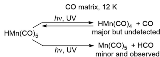
Scheme 8 Photochemistry of \text{HMn}(\text{CO})_5 in CO matrices.
