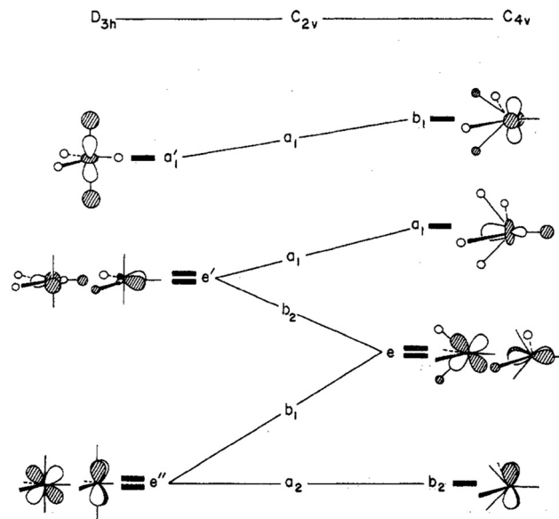
Fig. 13 Wave function and energy changes along a Berry pseudorotation for M(\text{CO})_5 . Reproduced with permission from Inorg. Chem. , 1975, 14 , 365–374. Copyright 1975, American Chemical Society. 116
