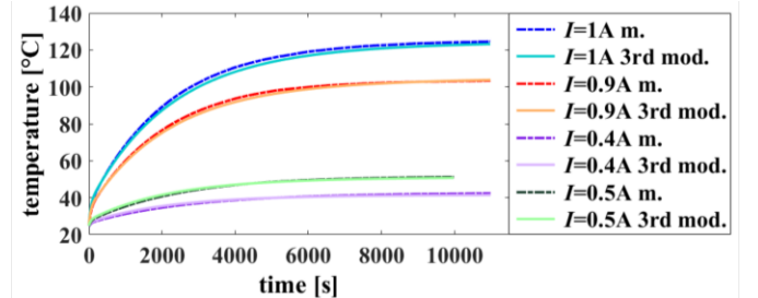
Fig. 9. Measured winding temperatures (m.) compared to the temperatures predicted by the 3 rd order analytical model for current I equal to 40, 50, 90 and 100% of the nominal current.
