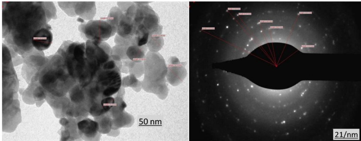
Fig. 4. TEM images of \text{LaFe}_{0.8}\text{Ti}_{0.2}\text{O}_3
