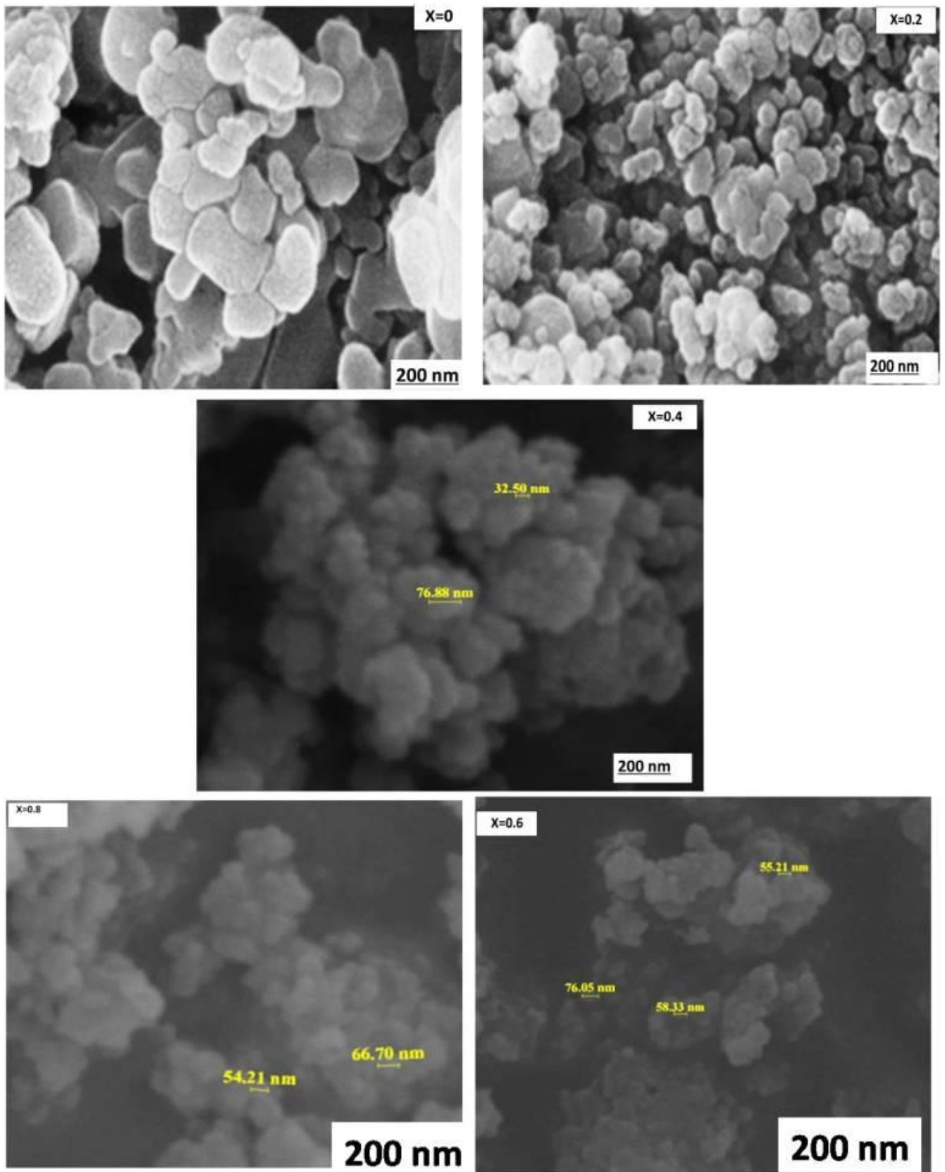
Fig. 2 SEM photographs of \text{LaFe}_{1-x}\text{Ti}_x\text{O}_3 ( x = 0, 0.2, 0.4, 0.6 & 0.8 )
