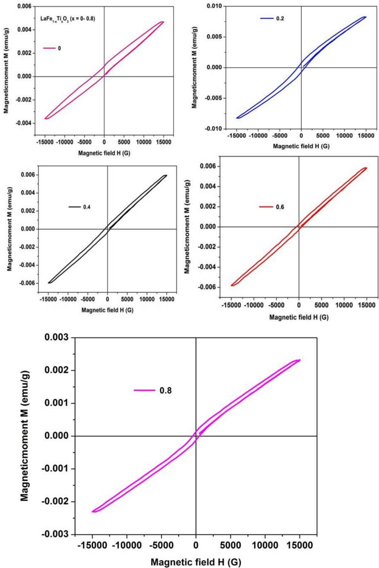
Fig. 7. VSM analysis of \text{LaFe}_{1-x}\text{Ti}_x\text{O}_3 ( x = 0, 0.2, 0.4, 0.6 & 0.8 )
