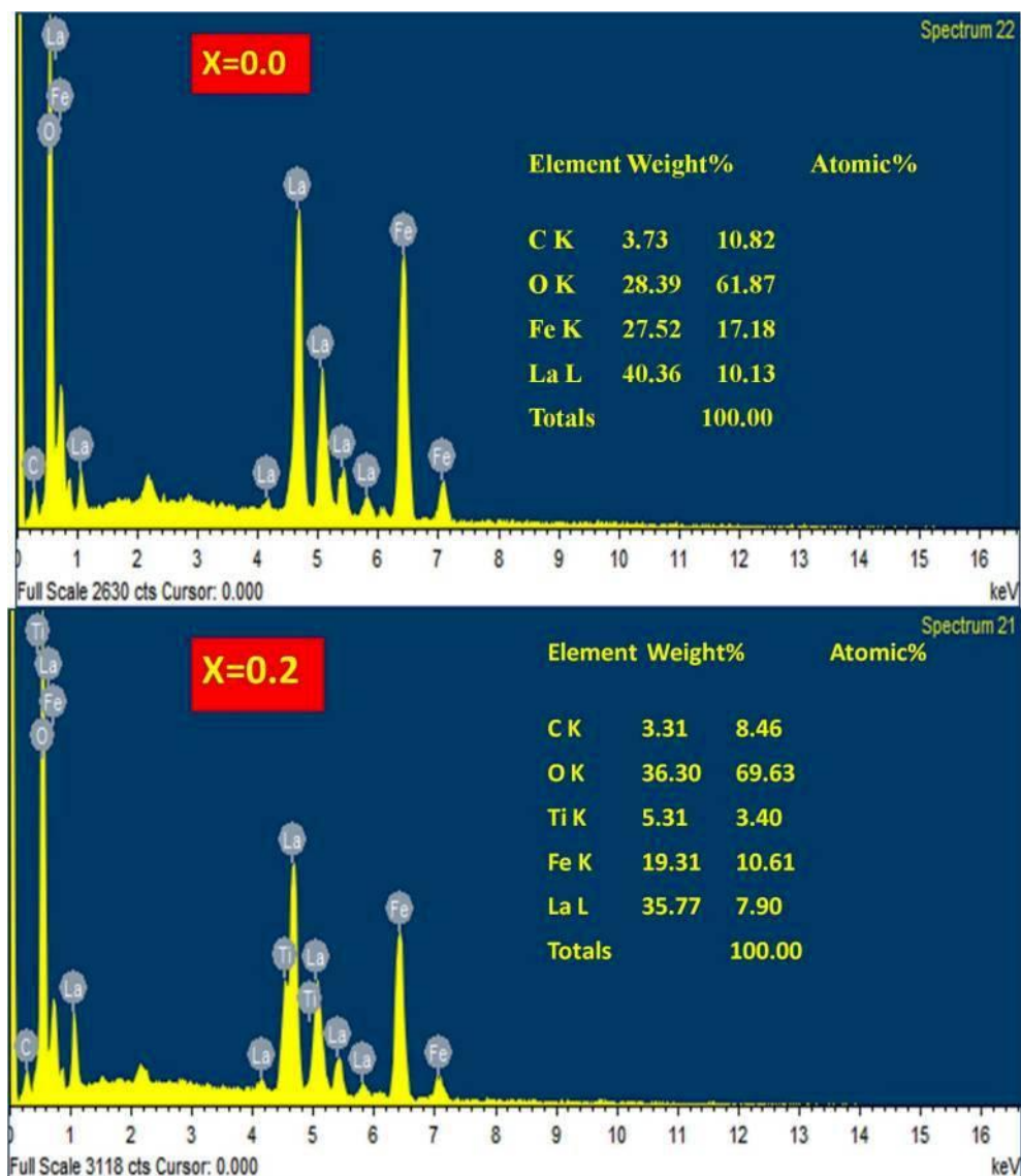
Fig . 3 EDAX spectra of \text{LaFe}_{1-x}\text{Ti}_x\text{O}_3 ( x = 0 & 0.2 )
