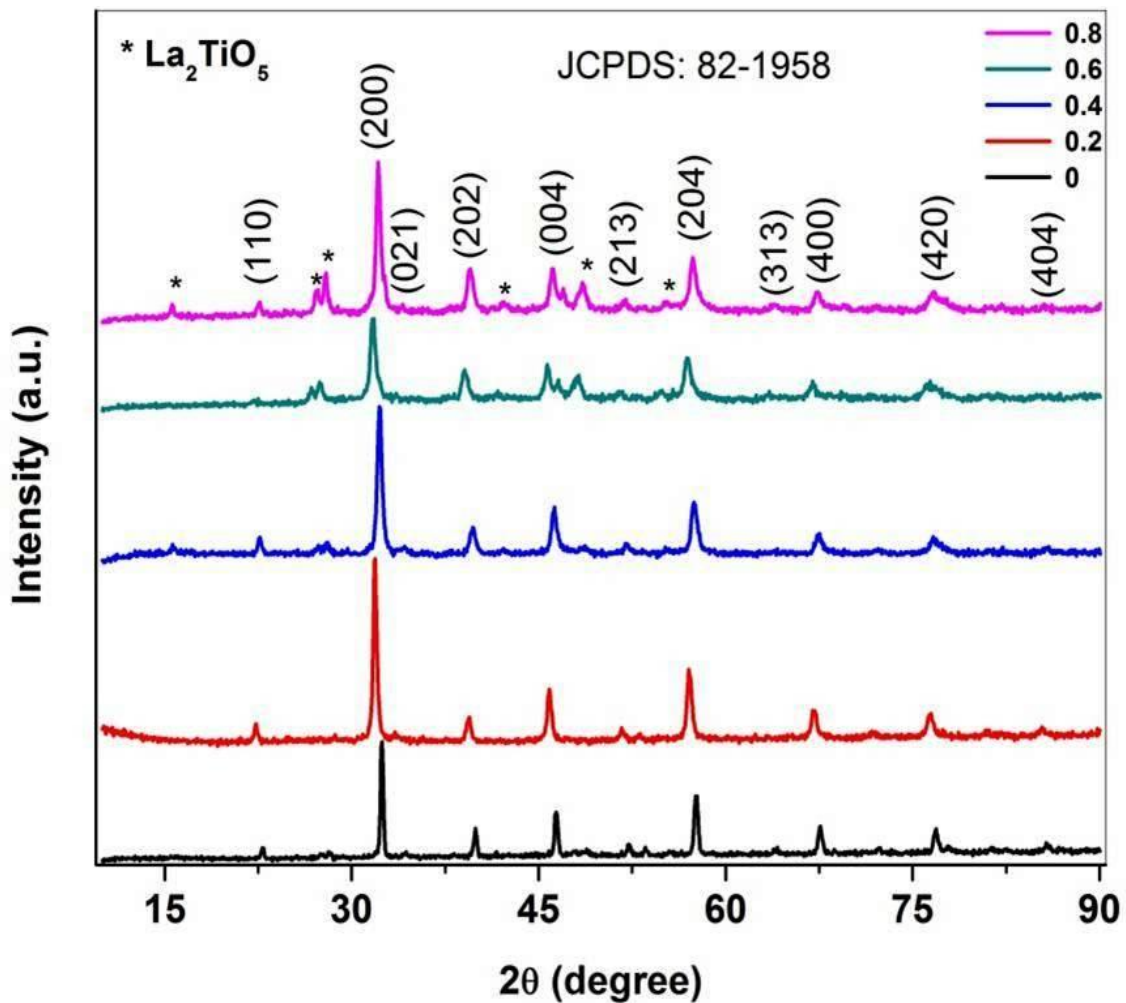
Fig. 1. XRD pattern of LaFe 1-x Ti x O 3 (x = 0.2, 0.4, 0.6 & 0.8)
