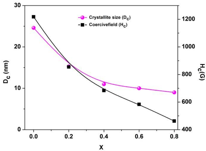
Figure.8. A graphical representation of dopant vs. coercivity and grain size of the nanopowders
