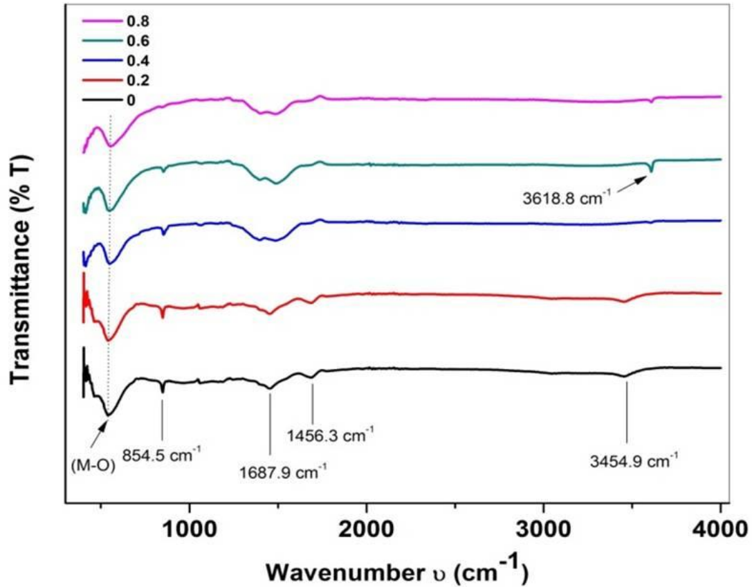
Fig.5 FTIR spectra of \text{LaFe}_{1-x}\text{Ti}_x\text{O}_3 ( x = 0, 0.2, 0.4, 0.6 & 0.8 )
