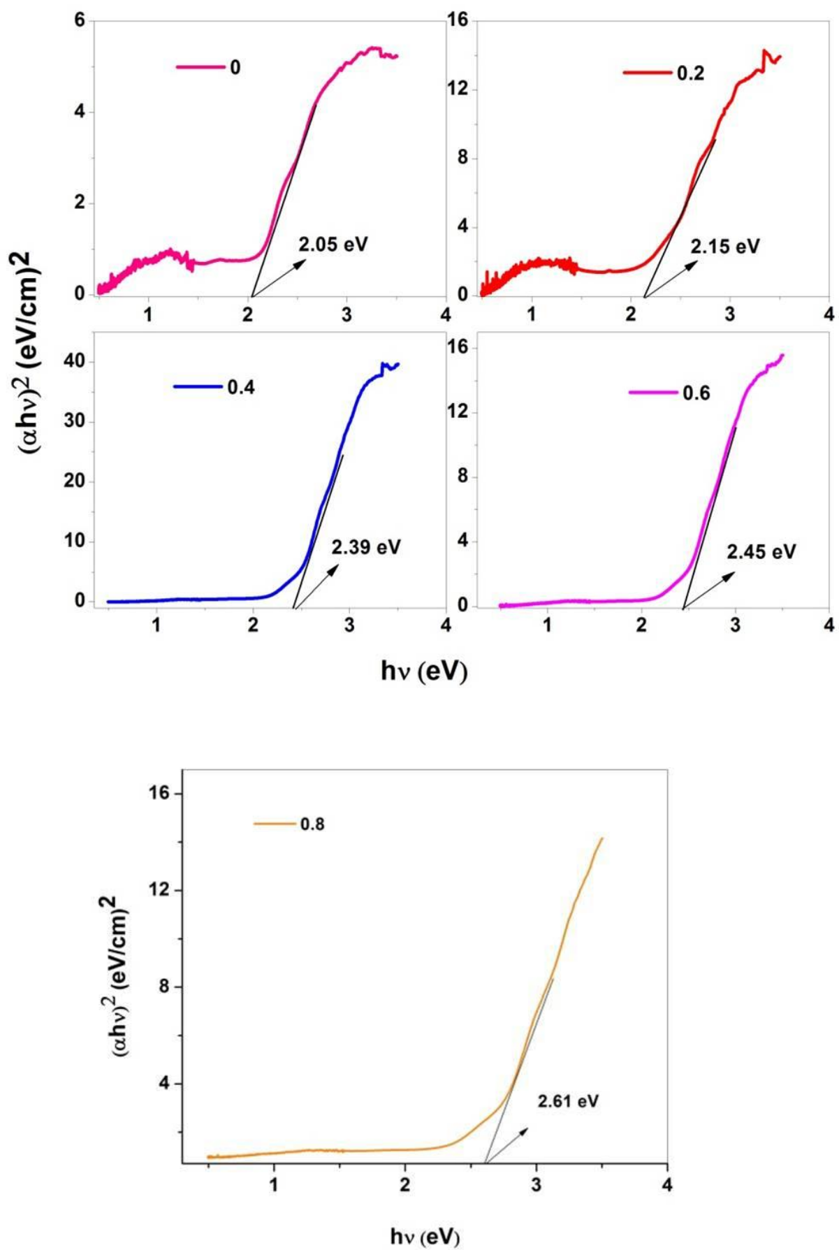
Fig. 6. UV-Visible spectra of \text{LaFe}_{1-x}\text{Ti}_x\text{O}_3 ( x = 0, 0.2, 0.4, 0.6 \text{ \& } 0.8 )
