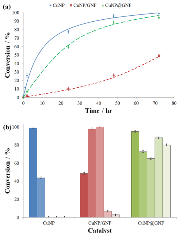
Figure 2. The comparative (a) kinetics and (b) recyclability over five cycles (measured as the conversion at 72 hr) for the copper catalysts dispersed in solution (CuNP), deposited on the surface (CuNP/GNF) or inserted in nanoreactors (CuNP@GNF).
