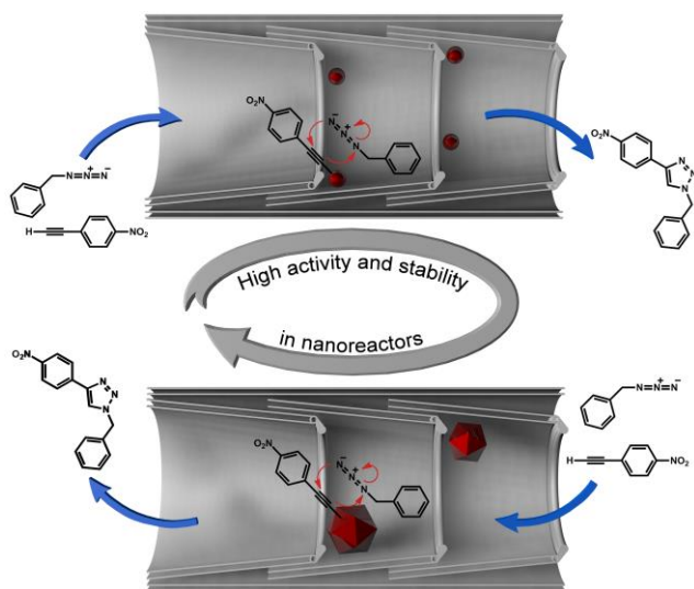
Scheme 1. The retention of high catalytic activity after multiple cycles using CuNP@GNF nanoreactor catalysts.
