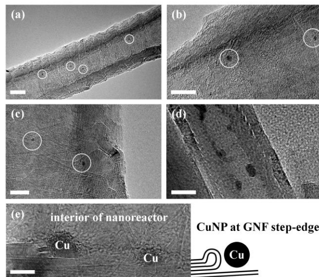
Figure 1. HR-TEM of CuNP@GNF. CuNP (~3 nm) immobilised at the step-edges (a-c) increase in size (~20 nm) following catalysis (d) or thermal treatment (e), but remain within the GNF inner channel. White circles guide the eye to the location of small 75 CuNP. Scale bars are 20 (a,d), 10 (b,c) and 5 nm (e).
