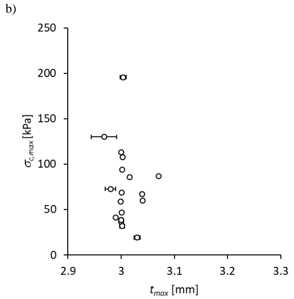
c) d) Figure 5. Maximum compaction stress, \sigma_{c,max} , and corresponding measured thickness, t_{max} , obtained with UTM thickness measurement for a) NCF dry, b) NCF wet, c) WOVEN dry and d) WOVEN wet.
