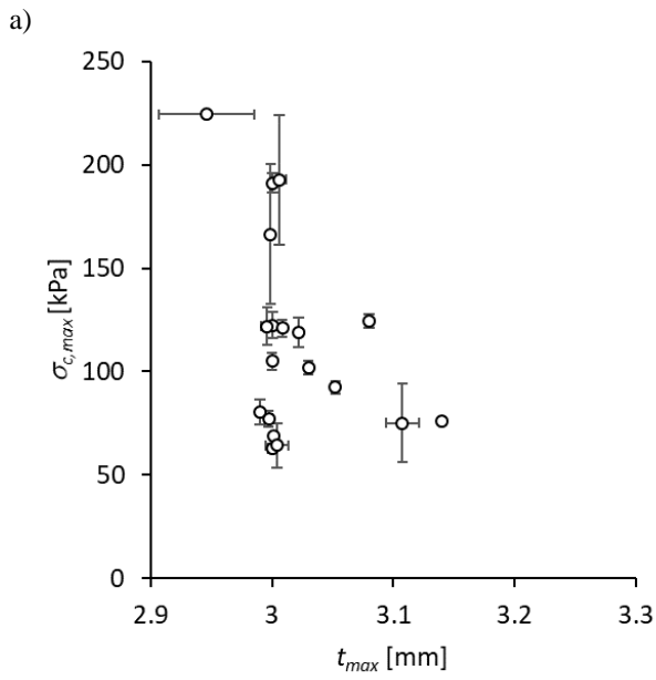
c) d) Figure 5. Maximum compaction stress, \sigma_{c,max} , and corresponding measured thickness, t_{max} , obtained with UTM thickness measurement for a) NCF dry, b) NCF wet, c) WOVEN dry and d) WOVEN wet.
