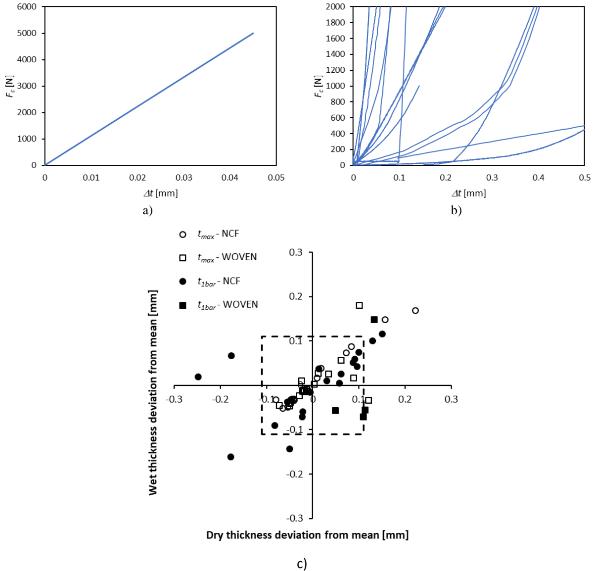
Figure 3. Machine compliance characterisation; a) Example of a compliance curve for a compression plate set-up on a universal testing machine; compaction force, F_c , is a linear function of apparent cross-head displacement, \Delta t . b) Compliance curves measured by different participants show a wide variety of dependencies of F_c on \Delta t . c) Specimen thickness (maximum and at 10^5 Pa of pressure) deviation from mean for dry and wet conditions compared to the average compliance reported by the participants. The dotted line box represents the average compliance \Delta t = 0.22 mm for an average compaction load F_c = 2700 N.
