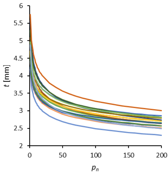
Figure 9. Fitted wet compaction curve for [thickness measurement source - material] a) [UTM - NCF wet], b) [LVDT/direct - NCF wet], c) [UTM - WOVEN wet] and d) [LVDT/direct - WOVEN wet].
