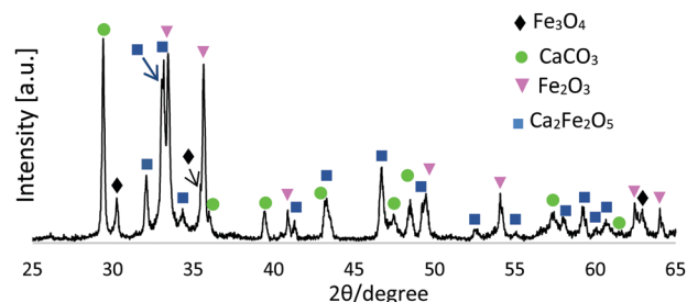
Fig. 1 XRD pattern for FS-processed \text{Fe}_3\text{O}_4\text{:CaCO}_3 .
