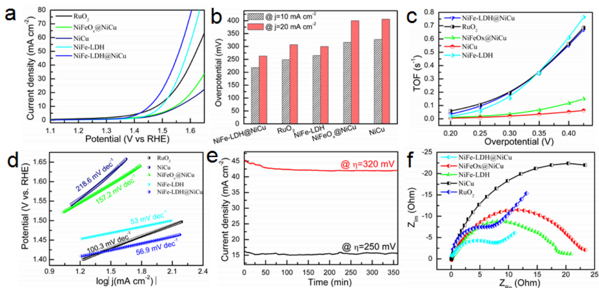
Fig. 3 OER performance of the catalysts in 1 M KOH. (a) Polarization curves recorded with a scan rate of 5 mV s -1 , (b) comparison of overpotentials at current densities of 10 and 20 mA cm -2 , (c) TOF as a function of overpotential, (d) corresponding Tafel plots, (e) Time dependence of current densities at overpotentials of 250 and 320 mV, and (f) Nyquist plots recorded at an overpotential of 300 mV.
