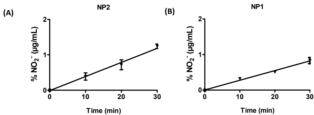
Figure S3. NO photorelease by Griess assay from NP2 (A) and NP1 (B) at the concentration of 0.2 mg/mL.
