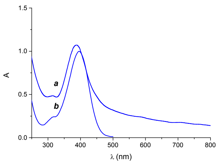
Figure S2. Absorption spectrum of NP2 (a) and, for comparison the free NOPD (b) in water.
