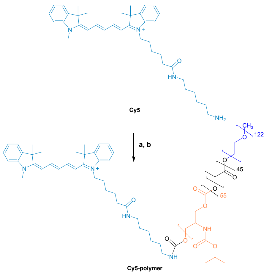
Scheme S1. Synthesis of Cy5-polymer. Reagents and conditions: a) DSC, TEA, CH 3 CN, 0 °C; b) protected polymer, TEA, CH 3 CN, 0 °C.
