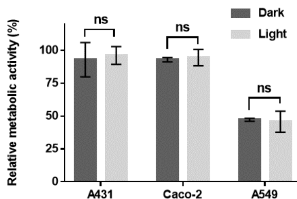
Figure S11. NP3 effect potency. Cells were exposed to NP3 for 48 hours either in the dark or under irradiation ( \lambda = 400 nm, 7 mW \text{cm}^{-2} , for 10 min). Metabolic activity was assessed using the PrestoBlue assay. Data represents the mean \pm S.D. (n=3).
