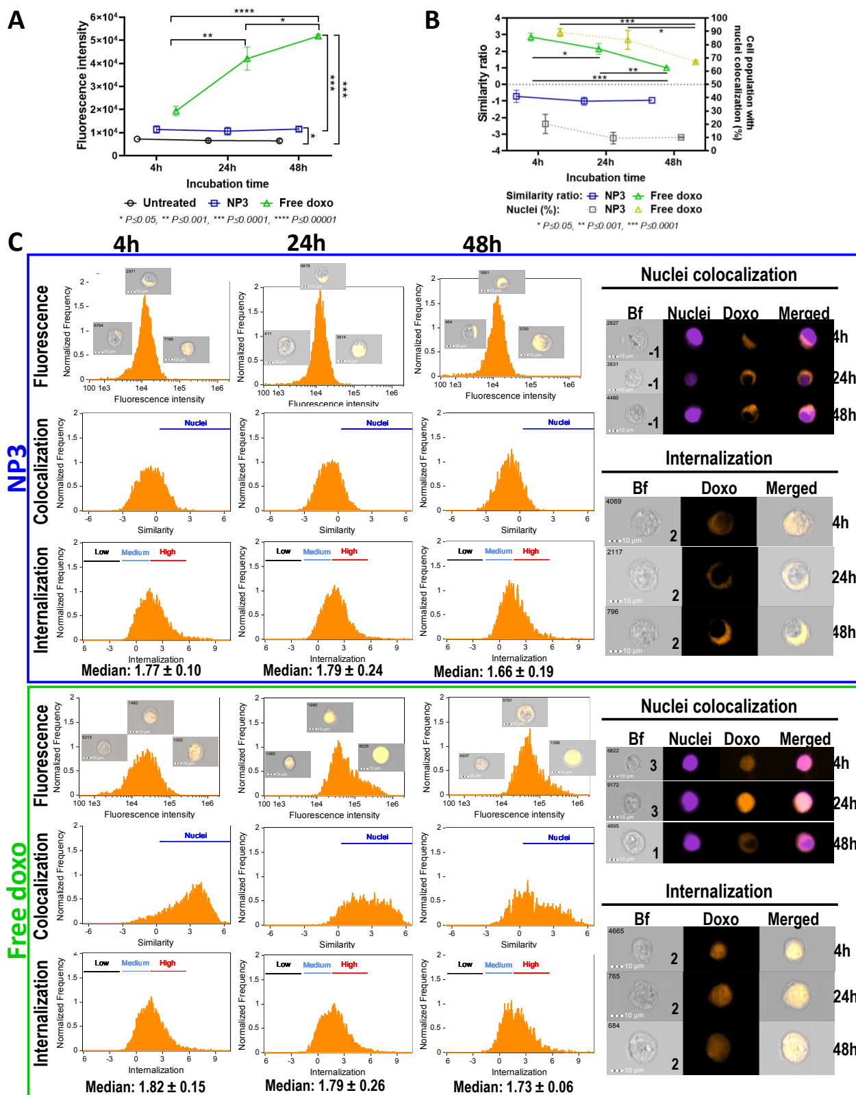
Figure S9. Median doxorubicin fluorescence intensity of NP3 and free drug at increasing time points (A). Ratio of doxorubicin nuclei colocalization with Hoechst nuclei dye and percentage of cells with positive nuclei colocalization (B). Caco-2 cells were incubated with NP3 and free drug at 1 \mu M doxorubicin for 4/24/48h (n=3). Representative images of nuclei colocalization and internalization and histograms of doxorubicin fluorescence intensity, colocalization and internalization for 4, 24 and 48h incubation times. Data was acquired in a ImageStream Flow Cytometer and analysed using IDEAS software (v. 6.2, Amnis).
