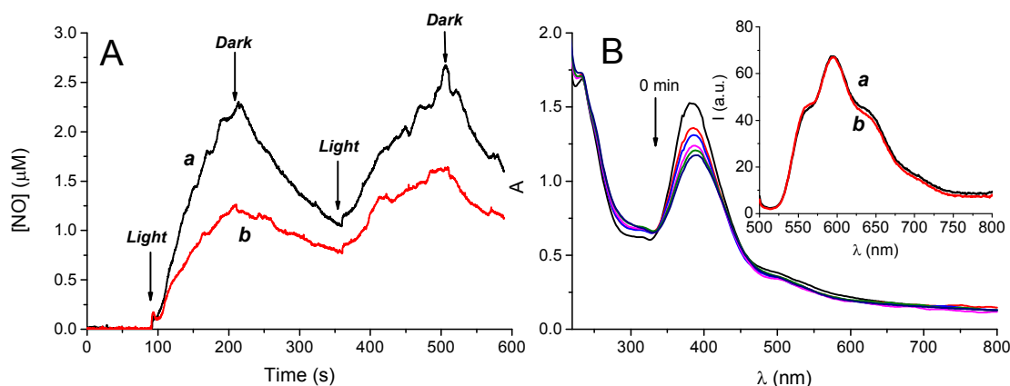
Figure 3. (A) NO release profile observed for water suspensions of NP2 ( a ) and NP1 ( b ); T = 25\text{ }^{\circ}\text{C} ; \lambda_{\text{exc}} = 405\text{ nm} . (B) Absorption spectral changes observed upon 405 nm light irradiation of a water suspension of NP2 for irradiation intervals of 0, 4.5, 6, 7.5, 9 and 10.5 min. The inset shows the fluorescence spectra of the NP2 before ( a ) and at the end of the irradiation ( b ).
