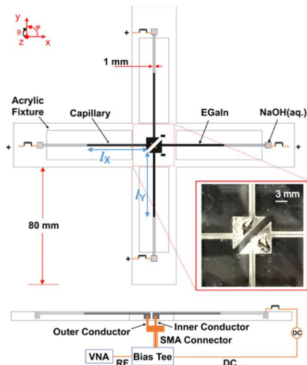
Fig. 23. Schematic of the reconfigurable crossed dipole antenna [151].
