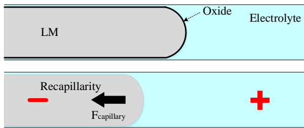
Fig. 2. Electrocapillarity method [22].
