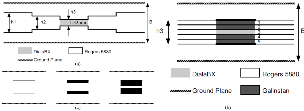
Fig. 12. Variable coupler using LM [66]. (a) Side view of a five-section wideband coupler. (b) Cross-section view of the middle section. (c) Different operating states of the coupler when different numbers of chambers are filled with LM.
