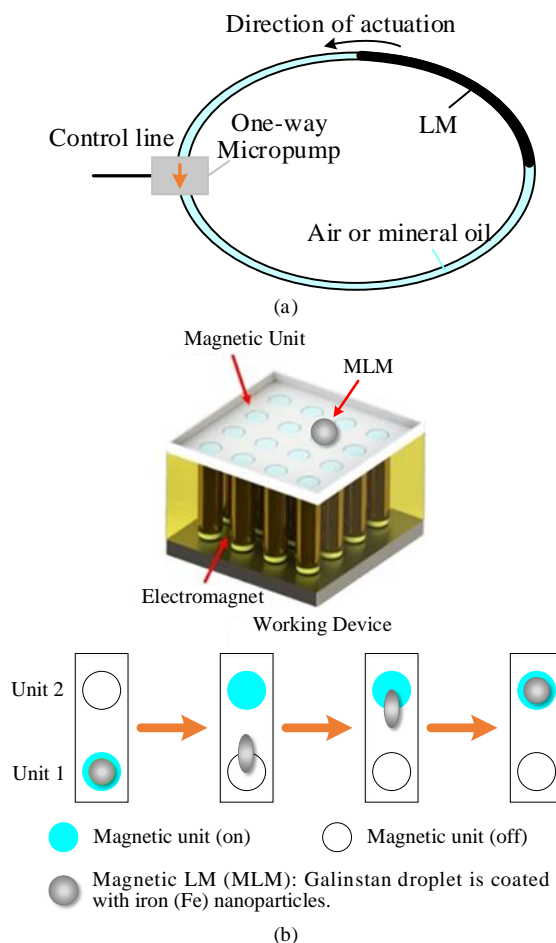
Fig. 1. Actuation of the LM: (a) Mechanical [12]. (b) Magnetic [19].
