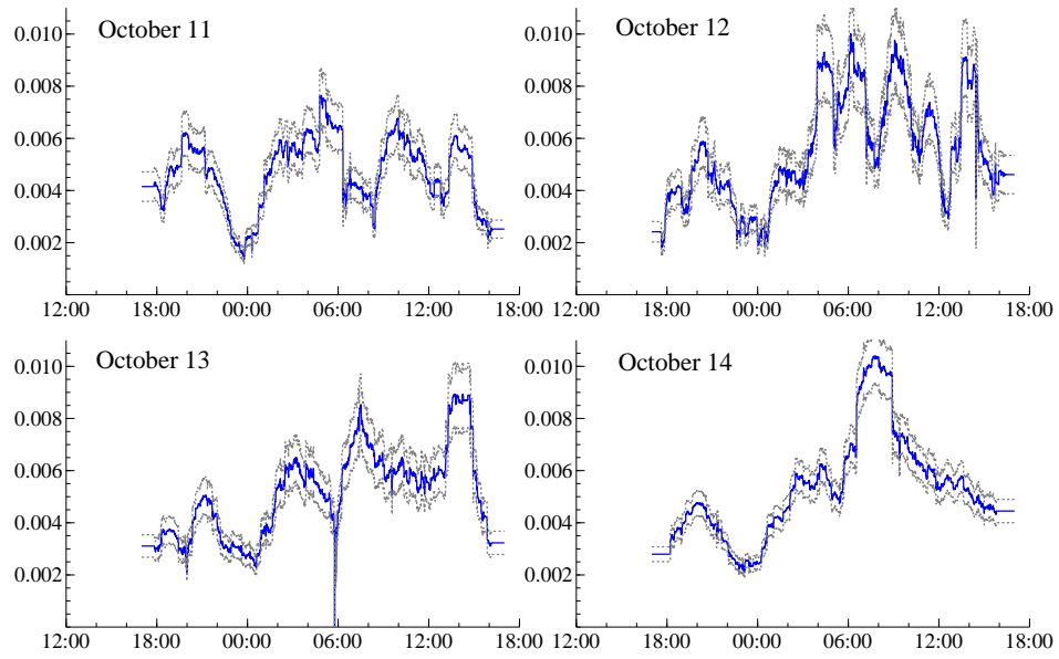
Figure 4: TSV with confidence interval, October 11–14, 2009
