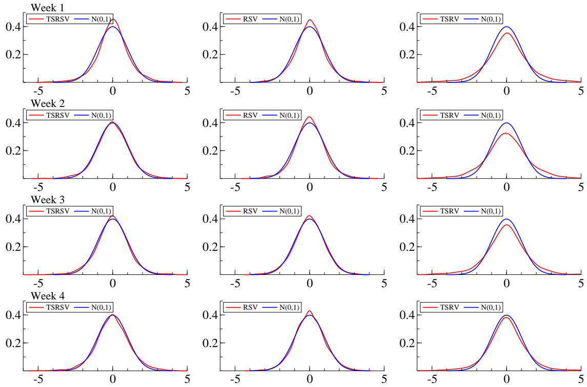
Figure 5: Densities of 3-minute returns standardized by TSRSV, RSV and TSRV, Week 1–4
