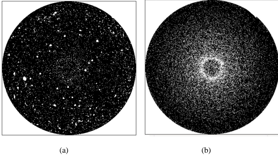
Fig. 6. X-ray CT scan of asphalt mastic stored at ambient temperature for four weeks suggests significant variation in mastic microstructural composition with depth. (a) bottom 2 mm of mastic. (b) top 2 mm. The lighter an image is, the more dense the material.
