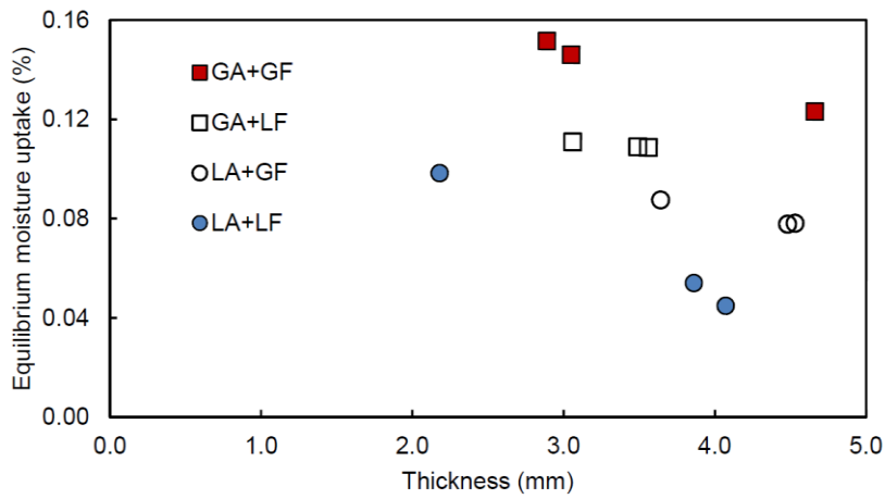
Fig. 2. Effect of aggregate and mineral filler type on asphalt mastic moisture uptake (243 hours conditioning time). For similarly sized mastics, moisture uptake in mastics containing granitic materials (aggregate and filler) is comparatively higher than the equivalent limestone containing mastics. GA = granite aggregate; GF = granite filler; LA = limestone aggregate; LF = limestone filler.
