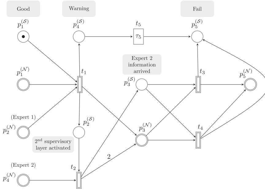
Fig. 8. Plausible Petri net of the example in Section 5.
