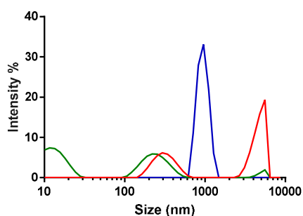
Figure 5. DLS traces in DI water of untreated 1 (red), PVPVA (green) and 1-PVPVA (blue) as a formulation. Light scattering measurements were collected on suspensions prepared with a final concentration of 0.5 mg/mL in drug (concentration adopted due to instrumental detection limits).
