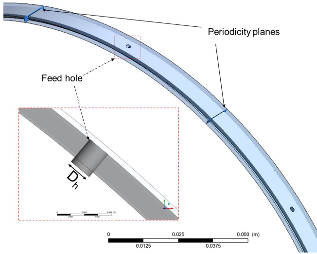
FIGURE 4: CAGE-INNER RACE PERIODIC GEOMETRY
