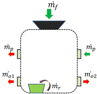
FIGURE 7: FLOW MONITOR
