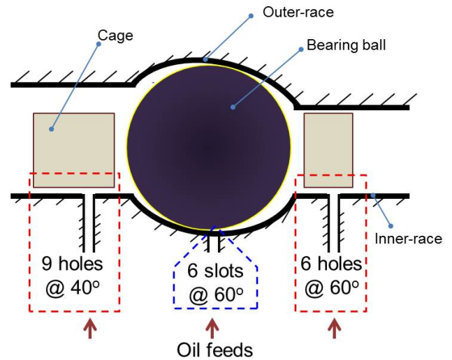
FIGURE 2: UNDER-RACE OIL FEED
