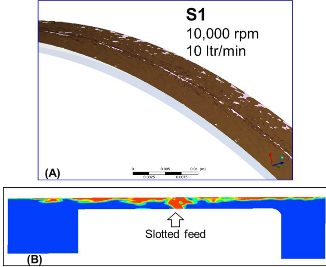
FIGURE 11: CAGE OIL WETTING FROM A SLOTTED FEED
