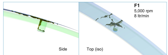
FIGURE 10: OIL BEHAVIOUR IN HOLE AND ON CAGE FOR 360° CASE
