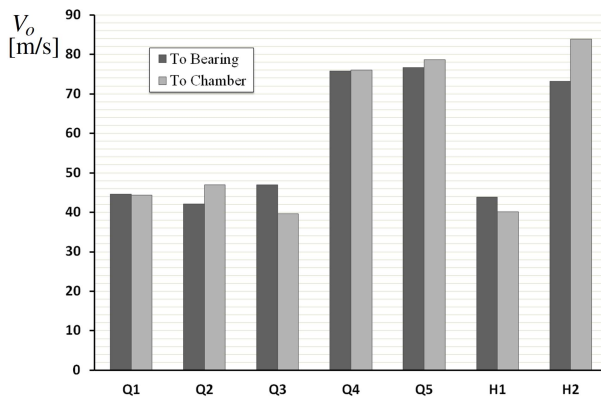
FIGURE 14: EXIT OIL VELOCITY
