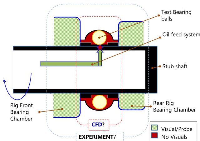
FIGURE 1: SCHEMATIC REPRESENTATION OF BEARING IN TEST FACILITY
