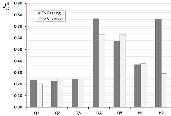
FIGURE 13: OIL EXIT SIZE FACTOR
