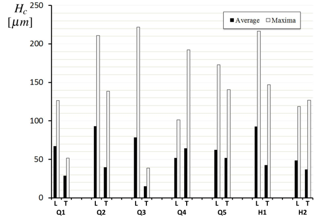
FIGURE 15: JET LEADING/TRAILING FILM THICKNESS
