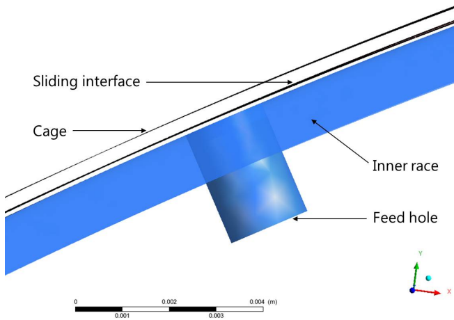
FIGURE 5: CAGE-INNER RACE FULL 360° ROTATING GEOMETRY
