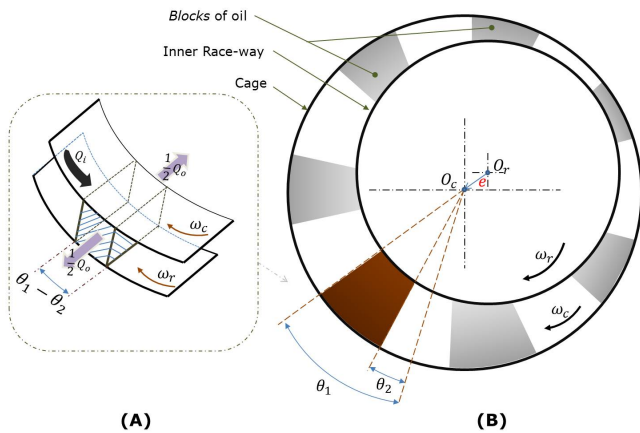
FIGURE 3: ILLUSTRATION OF THE MODEL OF ASHMORE ET AL [1] FOR AN OIL-FED CAGE-RACEWAY
