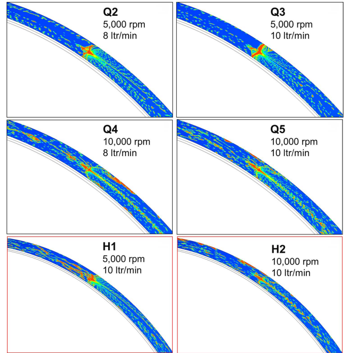
FIGURE 9: OIL WETTING OF THE CAGE FOR THE SECTOR MODELS
