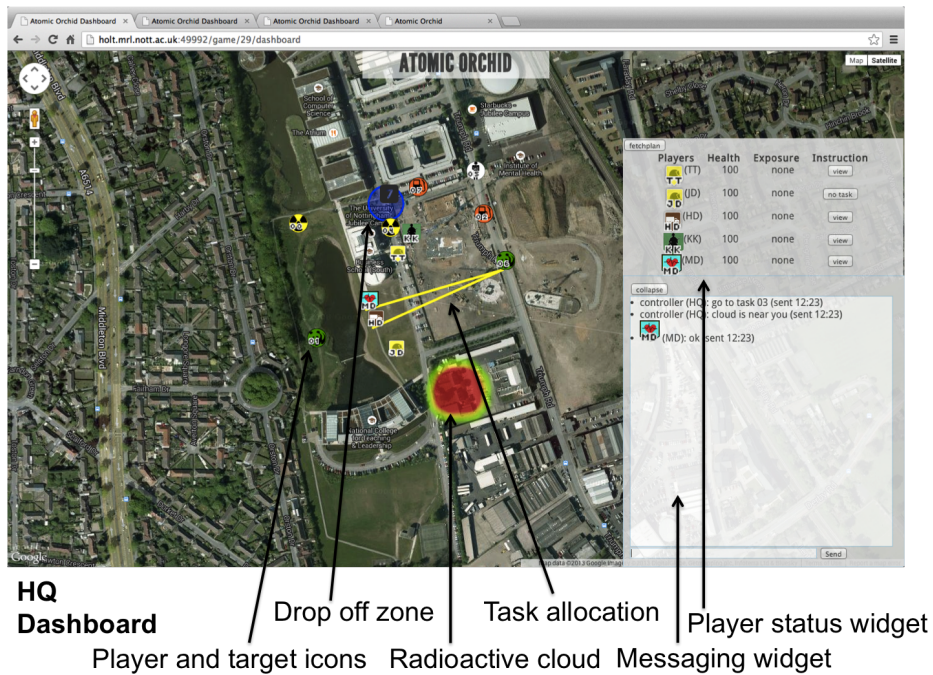
Fig. 2 HQ interface.
