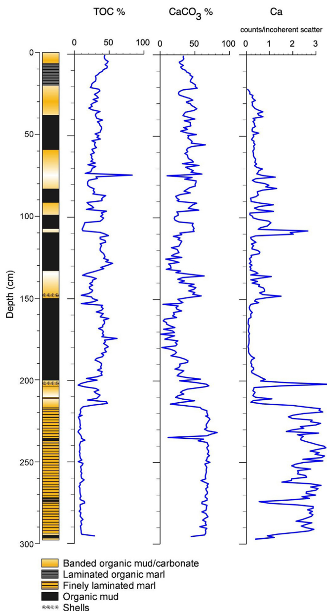
Fig. 3. Stratigraphy of the Yaal Chac core sequence (against depth), %TOC and % \text{CaCO}_3 based on LOI, Ca (counts/incoherent scatter).
