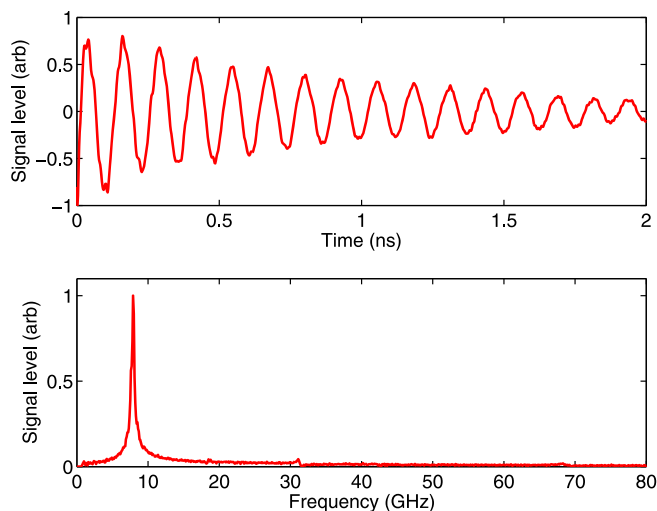
FIG. 11. (Color online) Experimentally measured time trace and spectrum obtained from a 5\ \mu\text{m} transducer fabricated with an intermediate PS layer between it and the substrate (compare with Fig. 5).
