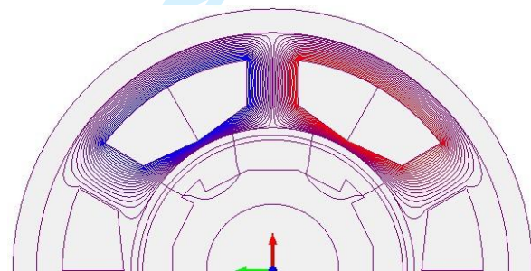
Fig. 9. Field lines distribution when only a phase is supplied
