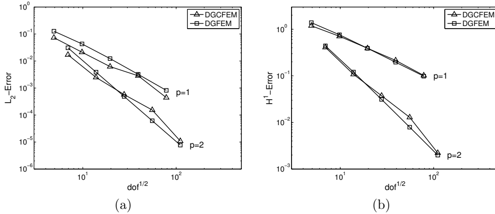
FIG. 9.3. Example 2. Comparison between the DGC FEM and the standard DGFEM (computed without any holes): (a) \|u - u_h\|_{L_2(\Omega)} ; (b) |u - u_h|_{1,h} .
