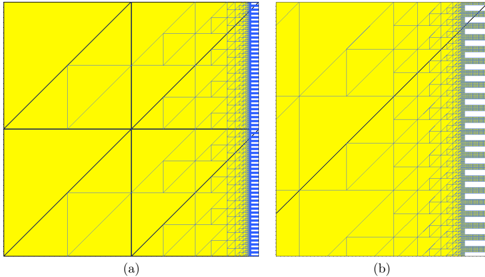
FIG. 9.1. Example 1: (a) Initial composite finite element mesh. The colour blue denotes elements present in the fine level mesh (which consists of 20160 triangular elements); elements plotted in black form the coarse level mesh (containing 8 elements); finally, the domain \Omega is shown in yellow. (b) Zoom of (a).
