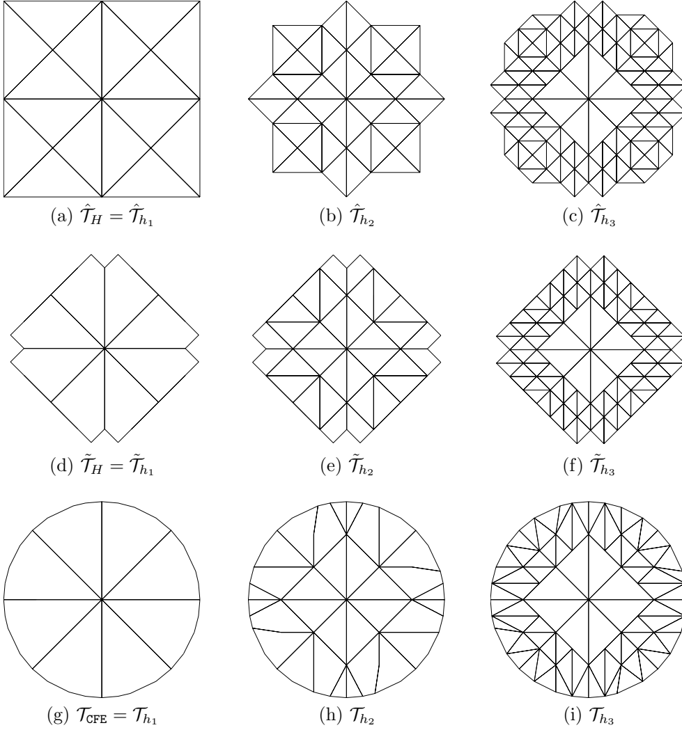
FIG. 3.1. Hierarchy of meshes: (a)–(c) Reference meshes; (d)–(f) Logical Meshes; (g)–(i) Corresponding physical meshes.
