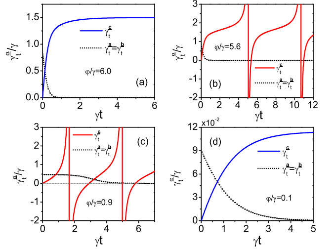
FIG. 1: Renormalized time-dependent rates [Eqs. (25) and (26)] corresponding to the multipartite trigonometric eternal non-Markovian evolution [Eq. (23)] for different values of the rate ratio \varphi/\gamma .
