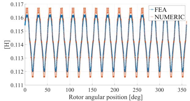
Fig. 6: L_{s_i s_i}(\alpha) : Stator self-inductance vs rotor angular position
