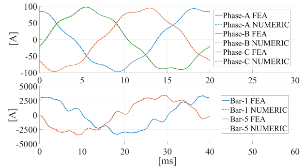
Fig. 15: Stator and rotor current waveforms: Slip = 0.5 [pu]
