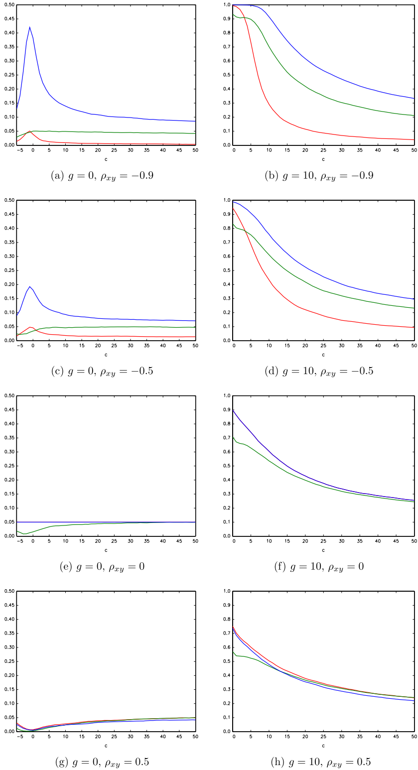
Fig. 1. Asymptotic size ( g = 0 ) and local power ( g = 10 ) of nominal 0.05-level tests based on the model in Eqs. (1)–(3) with innovation correlation \rho_{xy} ; \mathcal{T}_{con} : —, \mathcal{T}'_{con} : —, \mathcal{T}_N : —.
