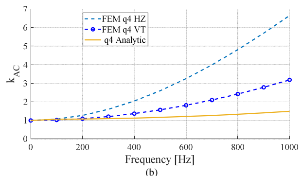
Fig. 6. Analytical Vs FEA results: a) Stator with q=2 , b) Stator with q=4 .
