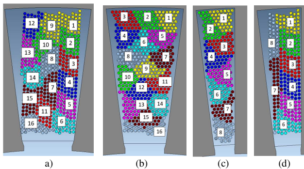
Fig. 3. Finite Element Models: a) q2_VT, b) q2_HZ, c) q4_VT, d) q4_HZ.
