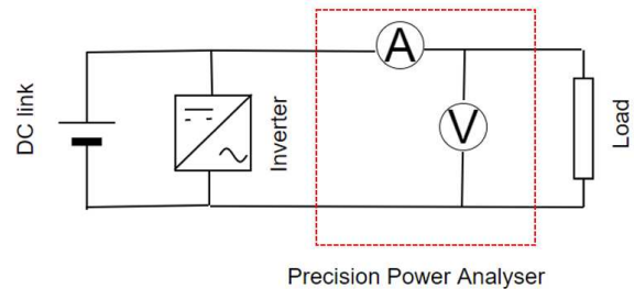
Fig. 12. PWM experimental setup and schematic layout.
