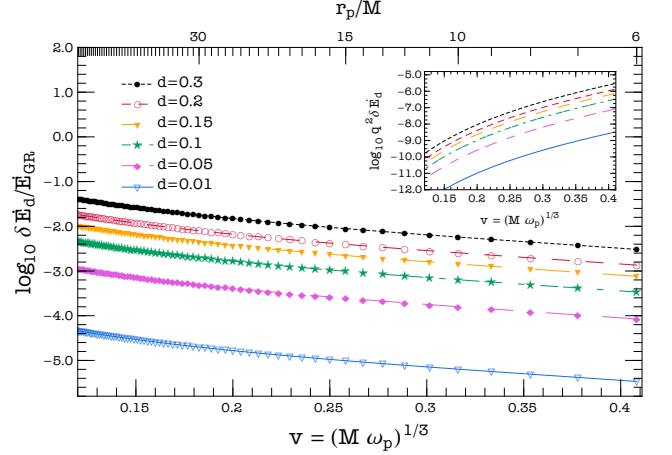
FIG. 1. Relative difference between the GW flux in modified gravity and in GR as a function of the orbital velocity v = (M\omega_p)^{1/3} (or radius r_p/M ), and of the scalar charge d . The inset shows the values of q^2 \delta\dot{E}_d .
