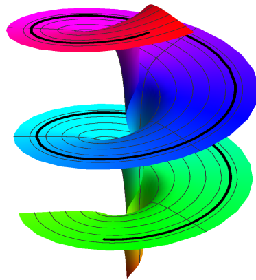
FIG. 1. The toy model potential V(\rho, \theta) given in (1) together with a typical inflationary trajectory indicated with the solid black line.
