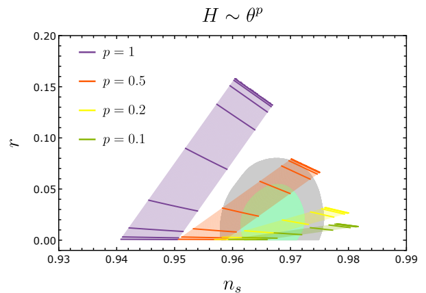
FIG. 2. The analytical predictions (12) for (n_s, r) compared to the Planck 1\sigma and 2\sigma contours [1]. We show the predictions for wavenumbers which cross the horizon 50 – 60 e-folds before the end of inflation. The predictions for n_s - r depend on the value of \kappa \in [1, 1000] , where the values (1, 2, 4, 8, 16, 32, 64, 128, 256) are depicted with thick lines (from bottom to top).
