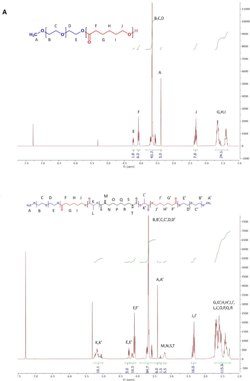
Fig. S2. ^1\text{H} NMR for P1 synthesis. (A) Diblock mPEG-PCL ( ^1\text{H} NMR (400 MHz, \text{CDCl}_3 ) \delta 4.27 – 4.19 (m, 2H), 4.07 (td, J = 6.7, 1.7 Hz, 6H), 3.85 – 3.42 (m, 44H), 3.38 (s, 3H), 2.40 – 2.27 (m, 8H), 1.72 – 1.32 (m, 24H)) and (B) P1 pentablock polymer ( ^1\text{H} NMR (400 MHz, \text{CDCl}_3 ) \delta 5.31 – 5.01 (m, 16H), 4.33 – 4.18 (m, 4H), 4.18 – 4.04 (m, 16H), 3.90 – 3.43 (m, 84H), 3.40 (s, 6H), 3.18 (d, J = 7.0 Hz, 6H), 2.39 – 2.25 (m, 16H), 1.74 – 1.19 (m, 116H))
