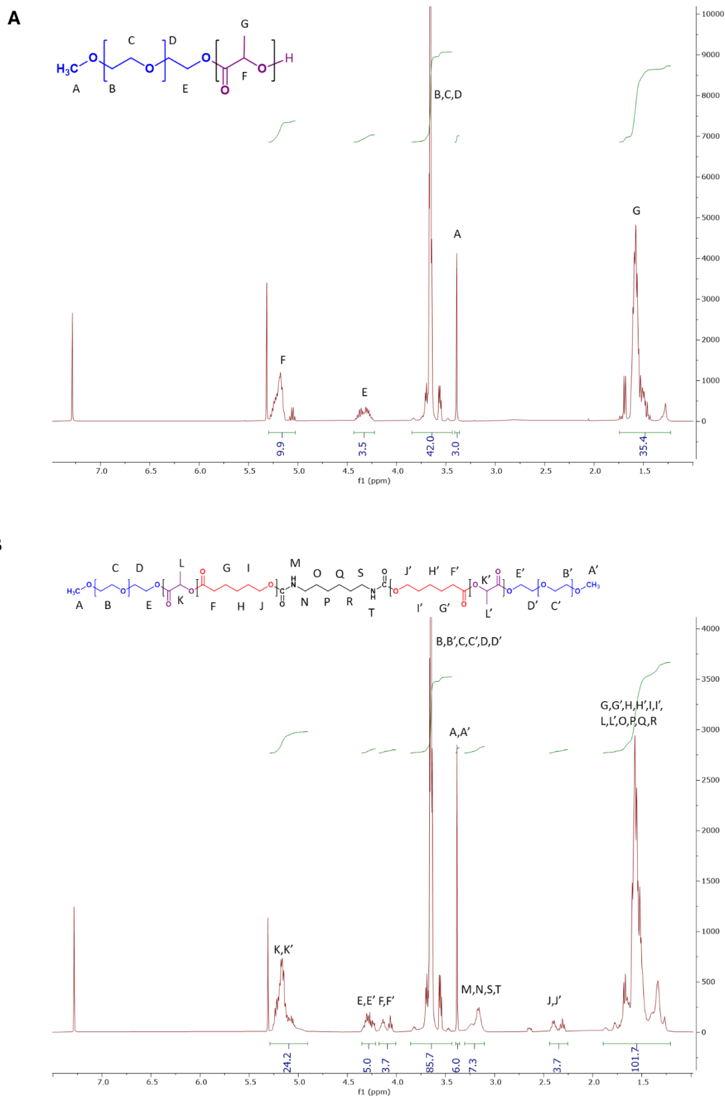
Fig. S7. ^1\text{H} NMR for P6 synthesis. (A) Diblock mPEG-PLA ( ^1\text{H} NMR (400 MHz, \text{CDCl}_3 ) \delta 5.25 – 5.02 (m, 10H), 4.35 (d, J = 6.7 Hz, 2H), 3.86 – 3.44 (m, 42H), 3.39 (d, J = 1.4 Hz, 3H), 1.59 (td, J = 7.3, 3.9 Hz, 36H)) and (B) P6 pentablock polymer ( ^1\text{H} NMR (400 MHz, \text{CDCl}_3 ) \delta 5.27 – 4.93 (m, 24H), 4.35 – 4.20 (m, 4H), 4.10 (dt, J = 31.2, 6.2 Hz, 4H), 3.86 – 3.44 (m, 86H), 3.38 (s, 6H), 3.17 (d, J = 6.9 Hz, 6H), 2.36 (dq, J = 33.8, 7.3 Hz, 4H), 1.89 – 1.23 (m, 102H)).
