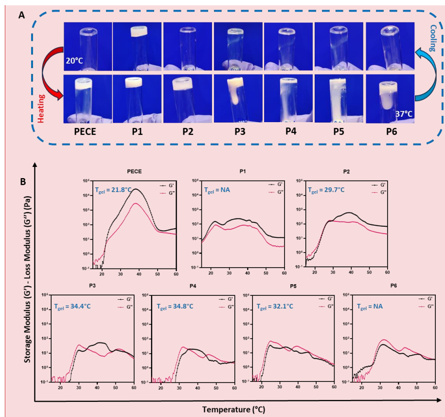
Fig. 1. Thermoresponsive Behaviour and Rheological Properties of Polymeric materials. (A) Tube inversion test as a proxy for rheological behaviour of the thermoresponsive polymers (30% w/v) at 20 °C and 37 °C. (B) Temperature-dependent changes in storage modulus ( G' ) and loss modulus ( G'' ) for polymeric materials (30% w/v), illustrating their rheological behaviour during the gelation process. ( T_{gel} = Gelation temperature, NA: Not applicable)
