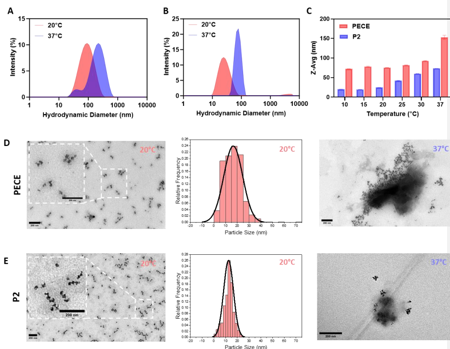
Fig. 2. Characterisation of thermo-responsive PECE and P2 NPs. Size distribution analysis of 1 % (w/w) of (A) PECE (20 °C: Z-avg = 75.7 nm, PDI = 0.221; 37 °C: Z-avg = 152.9 nm, PDI = 0.296) and (B) P2 NPs (20 °C: Z-avg = 24.9 nm, PDI = 0.207; 37 °C: Z-avg = 73.7 nm, PDI = 0.043). (C) Z-Avg (nm) differences between PECE and P2 NPs at different temperatures. Transmission electron microscopy (TEM) imaging and TEM size distribution analysis of (D) PECE and (E) P2 NPs at 20 °C (PECE: mean = 16.5 nm, PDI = 0.239; P2: mean = 12.5 nm, PDI = 0.112) and 37 °C (Scale bar = 200 nm).
