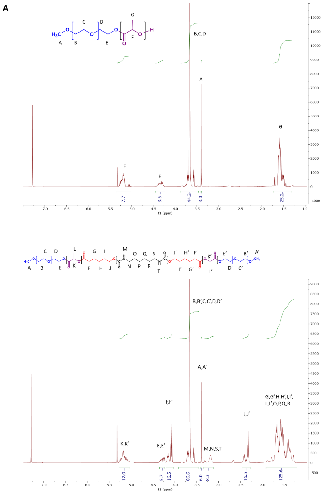
Fig. S3. ^1\text{H} NMR for P2 synthesis. (A) Diblock mPEG-PLA ( ^1\text{H} NMR (400 MHz, \text{CDCl}_3 ) \delta 5.29 – 5.09 (m, 6H), 4.44 – 4.23 (m, 3H), 3.86 – 3.46 (m, 13H), 3.40 (s, 3H), 1.73 – 1.32 (m, 24H)) and (B) P2 pentablock polymer ( ^1\text{H} NMR (400 MHz, \text{CDCl}_3 ) \delta 5.29 – 5.03 (m, 16H), 4.36 – 4.20 (m, 4H), 4.11 (dt, J = 31.1, 6.3 Hz, 16H), 3.90 – 3.44 (m, 86H), 3.39 (s, 6H), 2.48 – 2.28 (m, 16H), 1.90 – 1.16 (m, 126H)).
