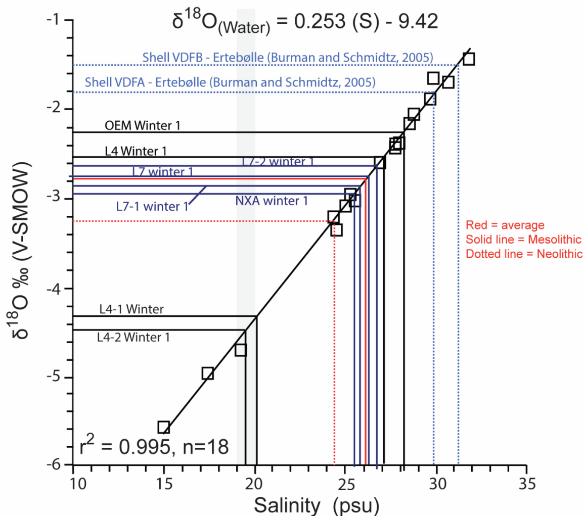
Figure S2. Modern relationship between salinity and \delta^{18}\text{O} (‰, SMOW) for the modern Limfjord water samples taken along a salinity gradient from Struer (average salinity=32 psu) in the western Limfjord to Klitgård (average salinity=20.2 psu) in the east. Modern water samples analysed by Burman and Schmitz (2005). A linear correlation was observed (shown here by the Limfjord mixing line) yielding a freshwater end member of -9.4 ‰ \delta^{18}\text{O} and an increase of +0.253 ‰ for each salinity unit. Following conversion of fossil shell winter \delta^{18}\text{O} in (VPDB) maxima to \delta^{18}\text{O} SMOW (step 2, Fig. S1), the salinity (at the 3.7^\circ\text{C} growth stop) for the Mesolithic and Neolithic sub-fossil shells was estimated using this relationship (see also Table S1). Source: Figure modified from Burman and Schmitz (2005).
