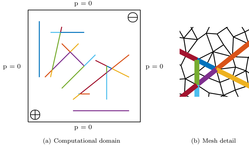
Figure 23: Example 3: Network of intersecting fractures: computational domain (left) and zoomed detail of the polygonal mesh employed for the computations (right). Taken from [17].
