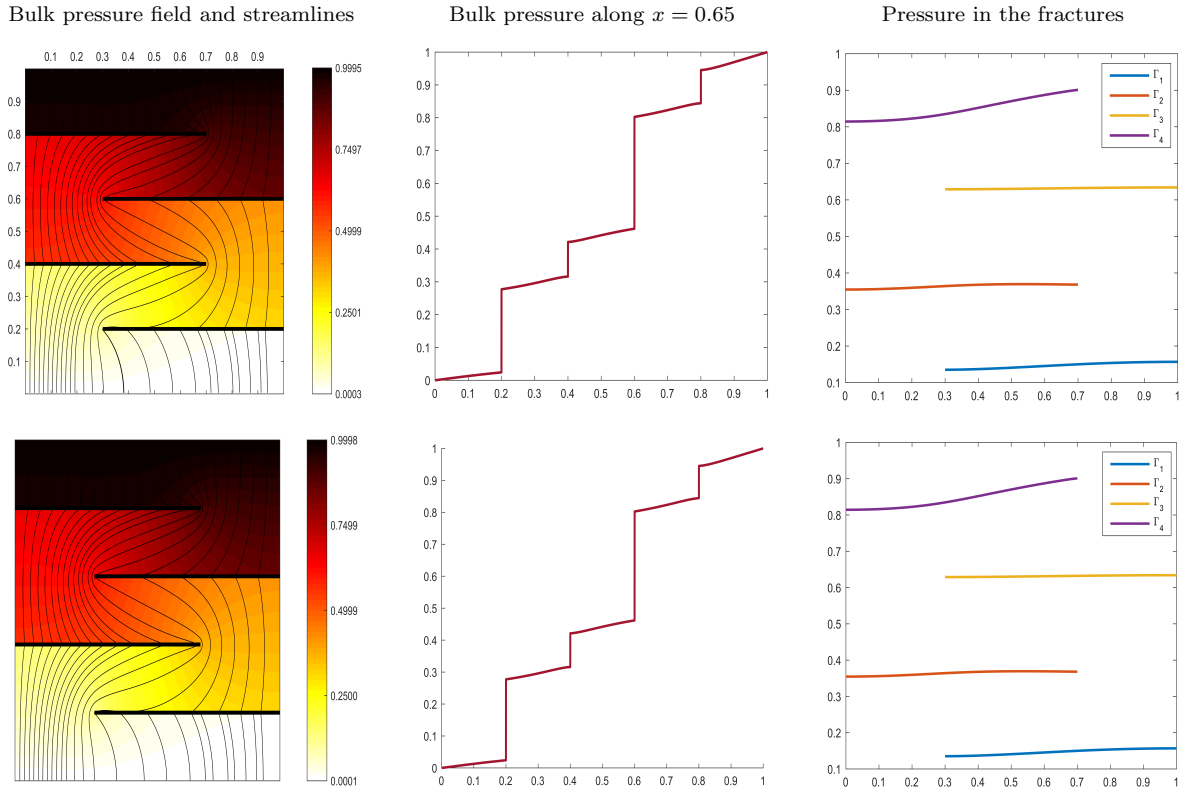
Figure 21: Example 2: Immersed fractures; configuration A, primal-primal approximation (top) and mixed-primal approximation (bottom).
