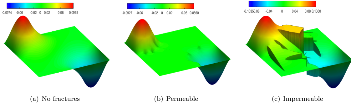
Figure 24: Example 3: Network of intersecting fractures: discrete pressure in the bulk for the three test cases, no fractures (left), permeable network \nu_{\Gamma}^{\tau} = \nu_{\Gamma}^n = 1000 (middle), impermeable network \nu_{\Gamma}^{\tau} = \nu_{\Gamma}^n = 0.001 (right). Taken from [17].
