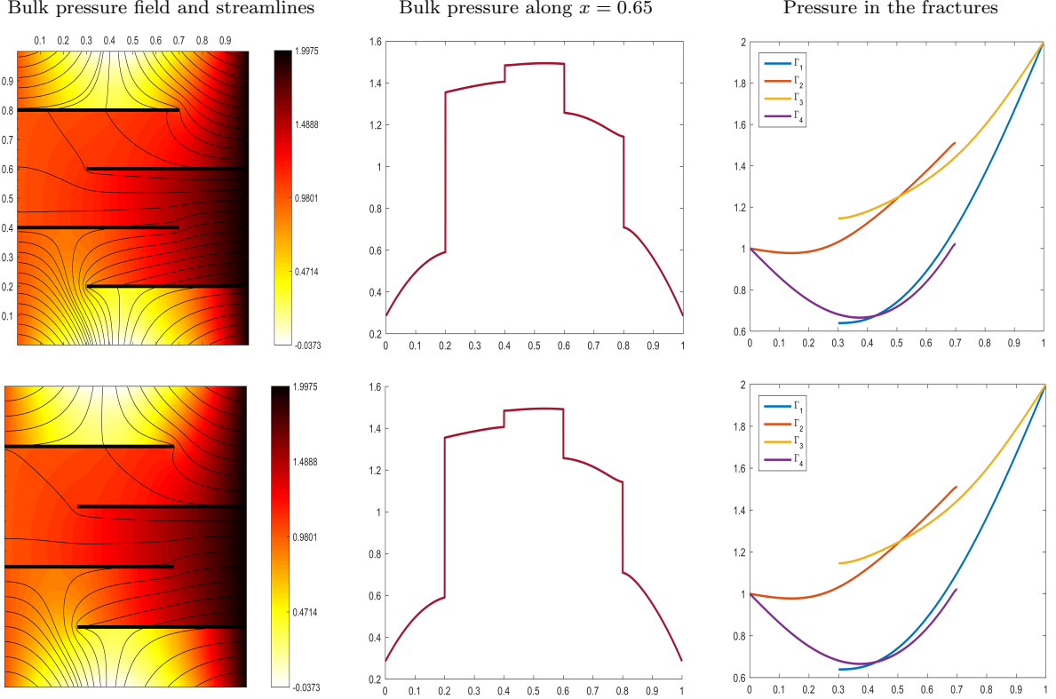
Figure 22: Example 2: Immersed fractures; configuration B, primal-primal approximation (top) and mixed-primal approximation (bottom).
