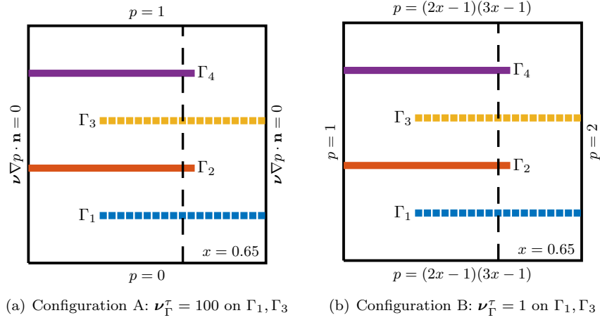
Figure 20: Example 2: Immersed fractures: configurations and boundary condition for the test cases A and B.
