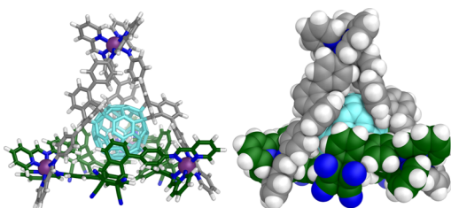
Figure 5. Two views of the MM3-optimized molecular model of [C_{60}\cdot 3] , based on the single-crystal X-ray structure of [C_{60}\cdot 1] . The TCNE-modified ligands are colored green.
