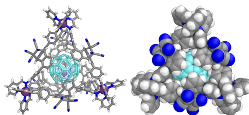
Figure 2. Two views of the cationic part of the crystal structure of [C_{60}C2] . Counterions, solvents, and disorder are omitted for clarity.
