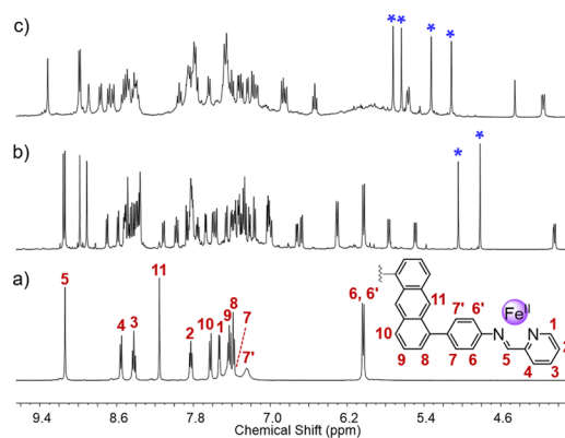
Figure 4. Partial ^1H NMR spectra (500 Hz, CD_3CN , 298 K) of (a) T -symmetric cage 1 , (b) C_3 -symmetric [C_{60}\cdot 1] , and (c) C_3 -symmetric [C_{60}\cdot 3] . The 9,10-dihydroanthracenyl protons of [C_{60}\cdot 1] and [C_{60}\cdot 3] are marked with blue asterisks.
