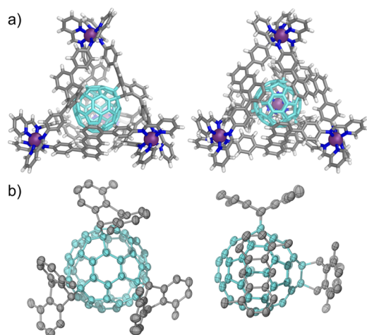
Figure 3. (a) Two views of the cationic part of the crystal structure of [C_{60}\cdot 1] . (b) Cutout of the tris(anthracenyl) C_{60} portion. Counterions and solvents are omitted for clarity.
