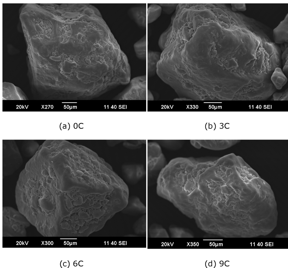
Fig. 9. SEM images of the PEI/silica adsorbents subjected to a certain number of TSA cycles with steam/N 2 regeneration.
