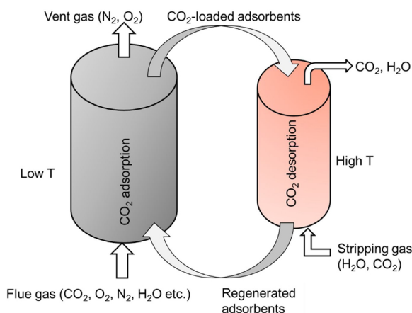
Fig. 1. Conceptual design of a solid adsorbent based CO 2 capture system using Temperature Swing Adsorption (TSA).
