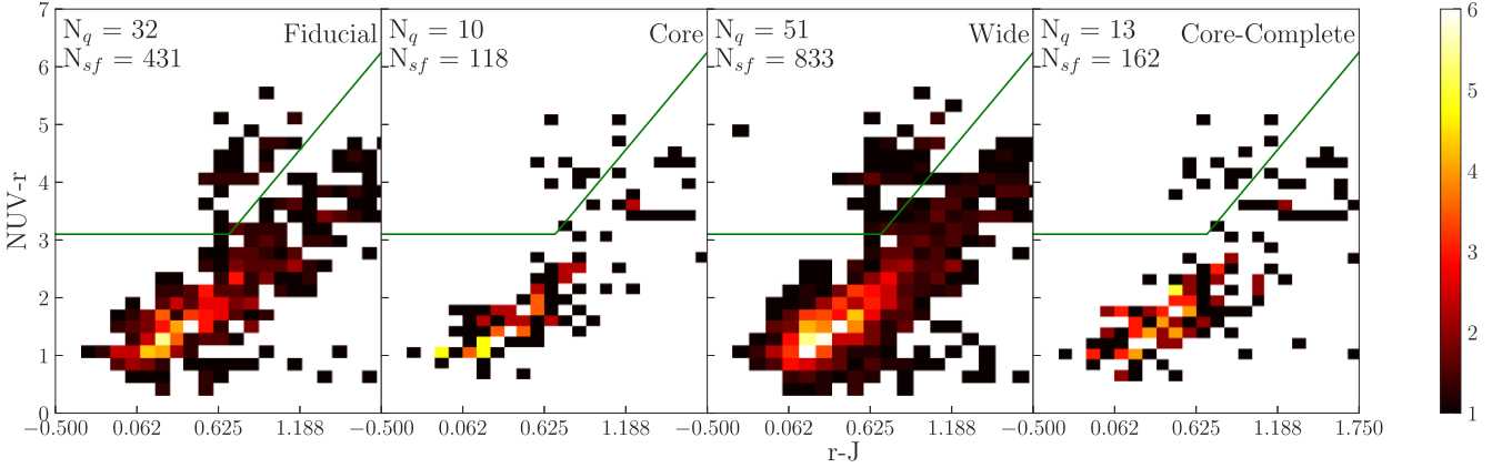
Figure B1. The (\text{NUV}-r) versus (r-J) colour distribution is shown for each volume selection (Table 3). The division between quiescent and star-forming galaxies is shown as the solid line. We observe a distinct quiescent population in each selection volume.
