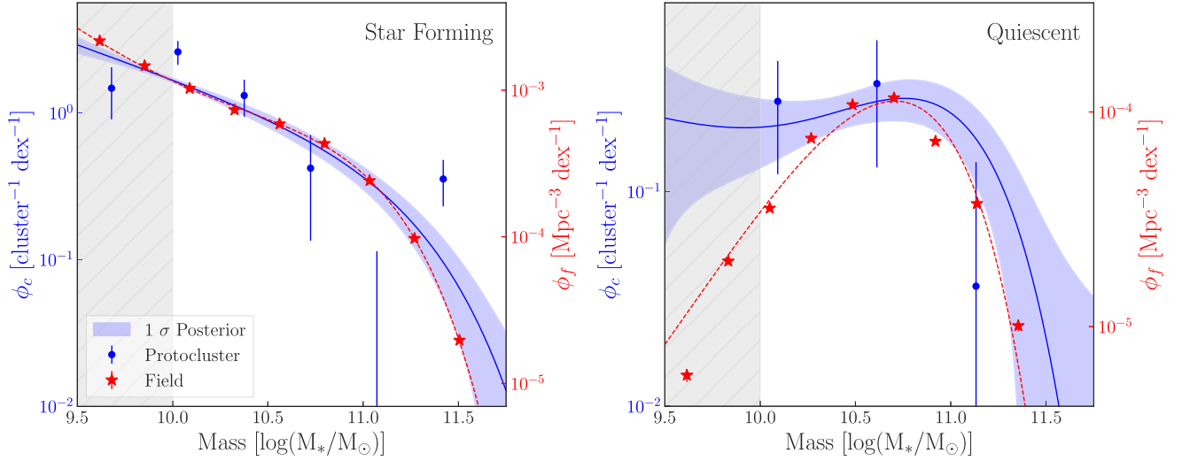
Figure B3. As Fig. 8, but for the core-complete sample ( dR = 0.5 \text{ Mpc} , dz = 0.3 ). Results are very similar to the core sample shown in Fig. B2. Uncertainties on the quiescent SMF are larger because the larger dz results in greater field contribution within the volume.
