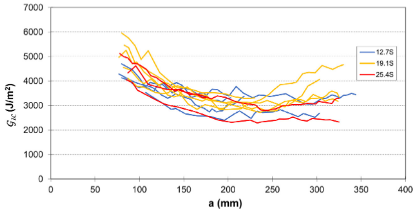
Fig. A.16. CBT-calculated fracture energy vs measured crack length plot for all DCB specimens.
