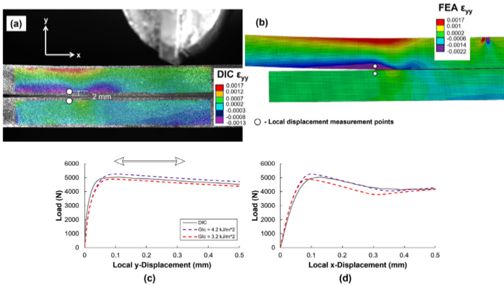
Fig. 14. (a) DIC and (b) FEA strain fields for a 12.75 SLB specimen and the corresponding plots for (c) load versus local y-displacement and (d) load versus local x-displacement for the specimen.
