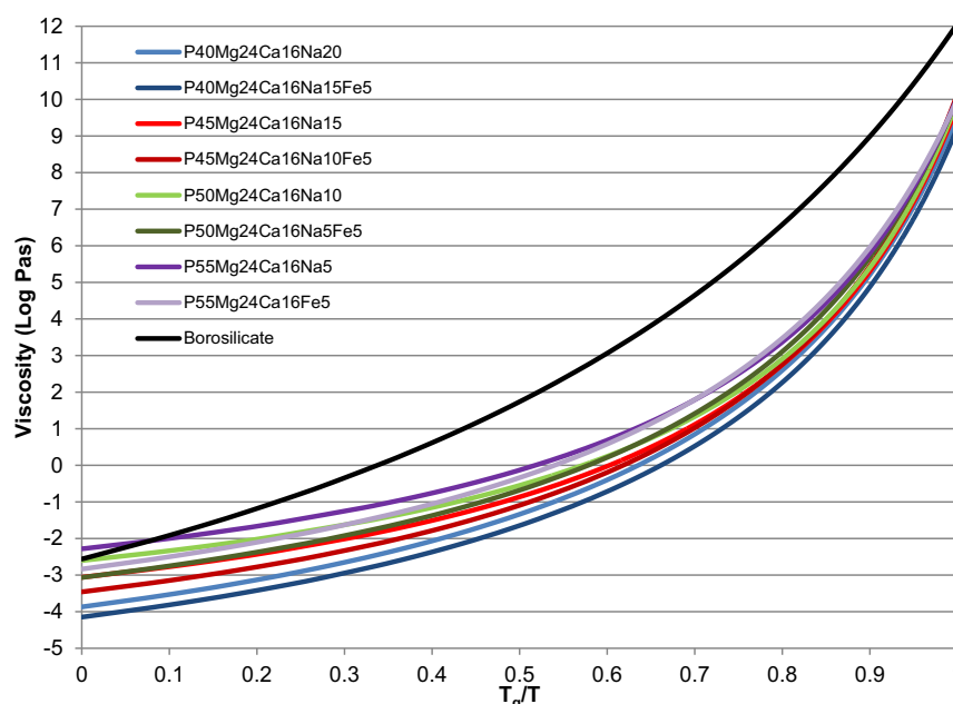
Fig. 8. Viscosity plotted against reduced temperature ( T_g/T ), with the standard glass for comparison. Errors are taken to be \pm 0.2 \text{ Log Pa}\cdot\text{s} .
