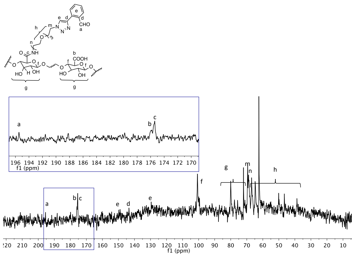
Figure S5- 13 C NMR of ALG ALD in DMF-d 7 at 25 C (120MHz).
