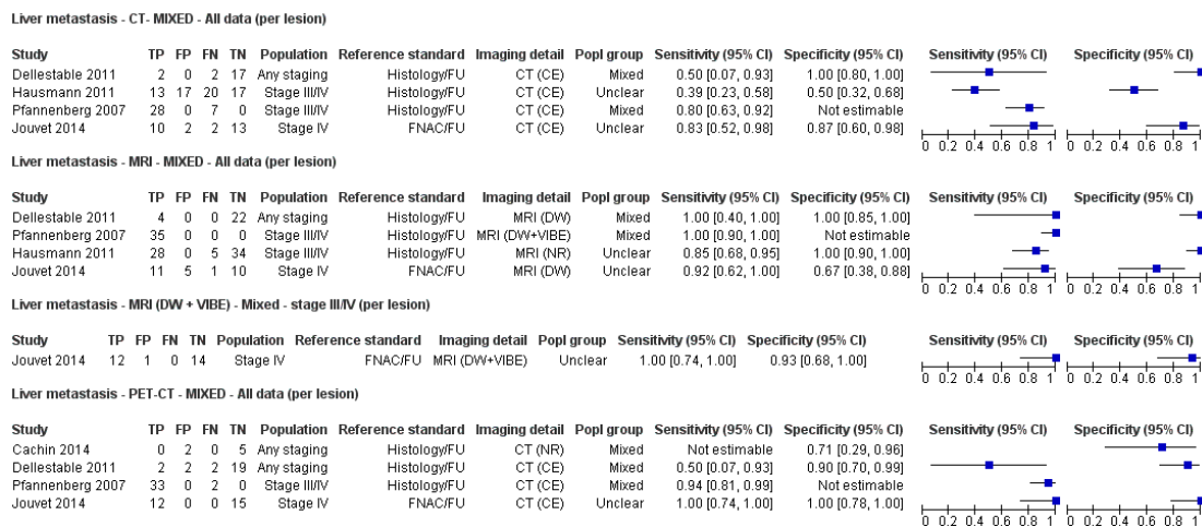
Figure 27. Forest plot of tests for the detection of liver metastasis in mixed population groups (per lesion data).
