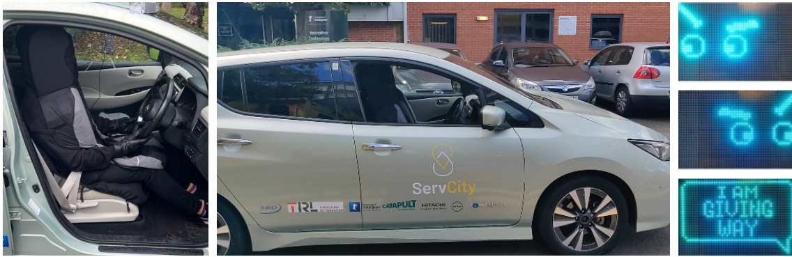
Figure 1: Driver in seat-suit (left); hidden driver operating car (centre); example eHMIs (right)
