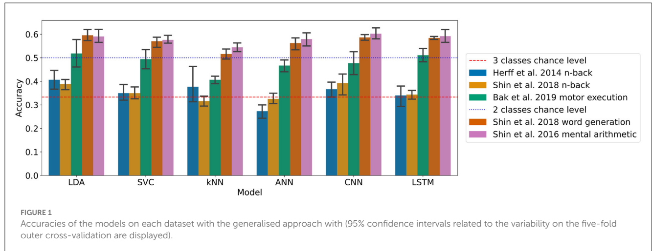
FIGURE 1 Accuracies of the models on each dataset with the generalised approach with (95% confidence intervals related to the variability on the five-fold outer cross-validation are displayed).
