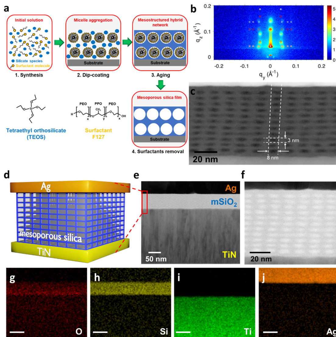
Fig. 1 Characterization of the 3D-structured mesoporous silica thin film and memristor. (a) Fabrication process of the sol-gel m\text{SiO}_2 thin films. (b) The GISAXS patterns of the m\text{SiO}_2 film with simulated Bragg peaks. The red circles and white squares represent the transmitted and reflected Bragg peaks, respectively. (c) Cross-sectional TEM image of the as-deposited mesoporous silica thin film. (d) Schematic of the m\text{SiO}_2 based memristor. (e) A cross-sectional TEM image of the m\text{SiO}_2 memristor. (f) Higher magnification TEM image of the m\text{SiO}_2 thin film in the memristor. (g–j) Cross-sectional TEM-EDX of the m\text{SiO}_2 based memristor. The scale bar is 50 nm.
