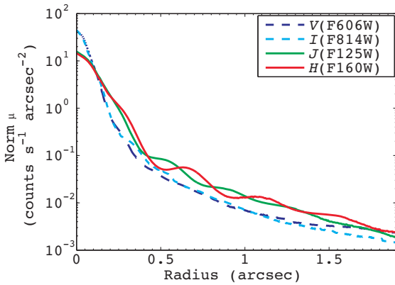
Figure 3. The CANDELS HST PSFs. Radial light \mu(r) profiles for the CANDELS PSFs, showing the differences in structure between the four wavebands. These PSFs have been empirically determined from isolated stars in the CANDELS HST images. All profiles have been normalized using the flux contained within a 2.828 arcsec aperture.
