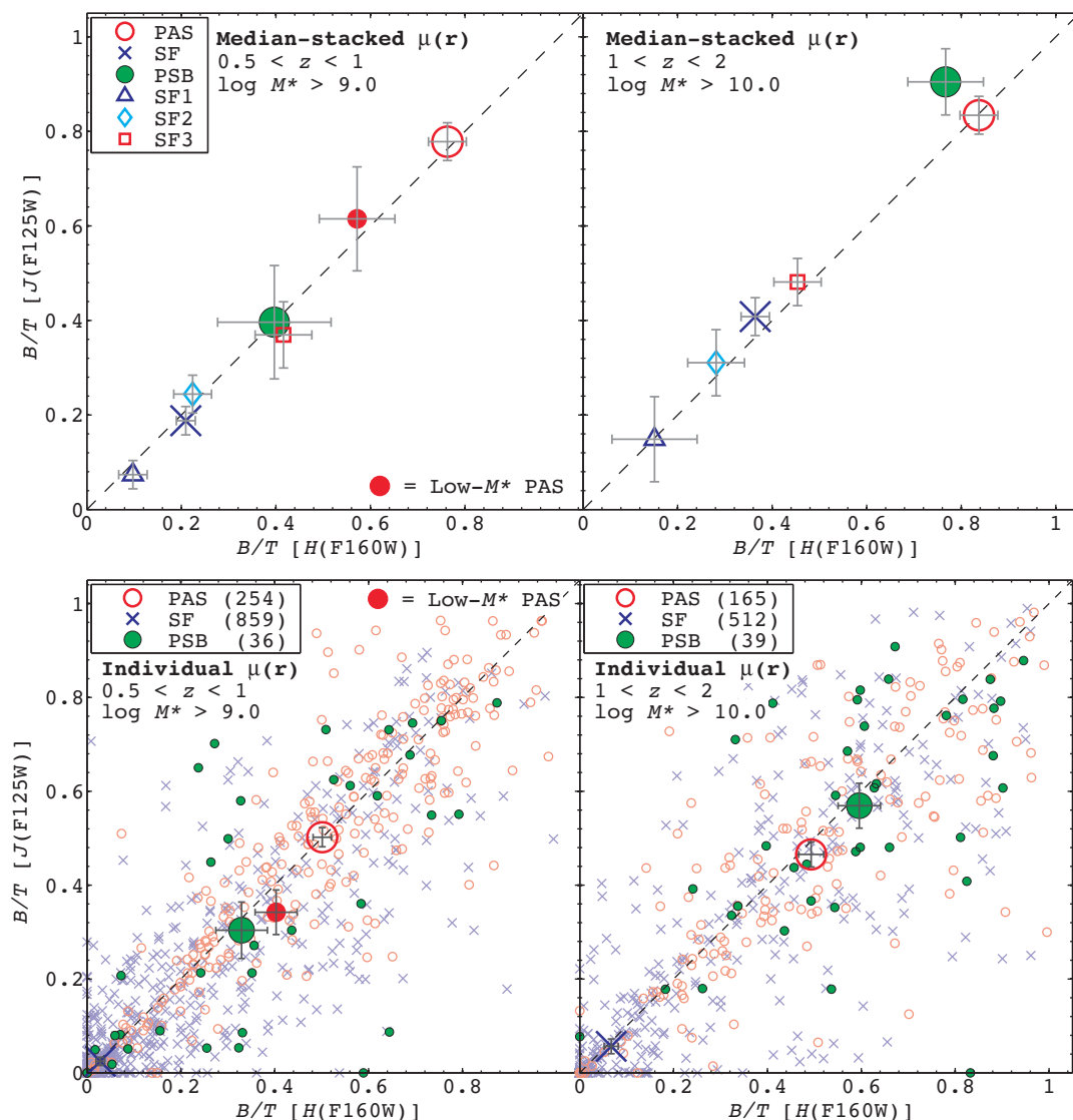
Figure 10. B–D decompositions for our galaxy populations at two epochs: 0.5 < z < 1 (left-hand panels) and 1 < z < 2 (right-hand panels). A comparison of the maximal B/T in J_{F125W} and H_{F160W} for the median-stacked light profiles \tilde{\mu}(r) (top panels), and for our individual \mu(r) profiles (bottom panels). In the bottom panels, large symbols represent the median B/T in each population, with associated 1\sigma errors. The typical B/T for the low-mass passive population ( 10^9 < M_* < 10^{10} M_\odot ) is also indicated. We find PSBs to exhibit significantly different structures at different epochs: bulge-dominated at 1 < z < 2 , but disc-dominated at 0.5 < z < 1 .
