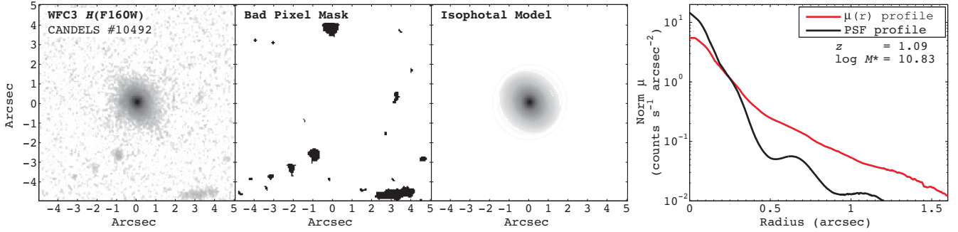
Figure 2. An example isophotal fit for a typical PSB galaxy. Left-hand panel: HST /WFC3 H_{F160W} image. Centre left-hand panel: the bad pixel mask used for the isophotal fit. Centre right-hand panel: the isophotal model generated by ellipse. Right-hand panel: the resultant azimuthally averaged radial light \mu(r) profile (red line), with the HST /WFC3 H_{F160W} PSF profile (black line) also shown for reference. Both profiles have been normalized using the flux contained within a 2.828-arcsec aperture.
