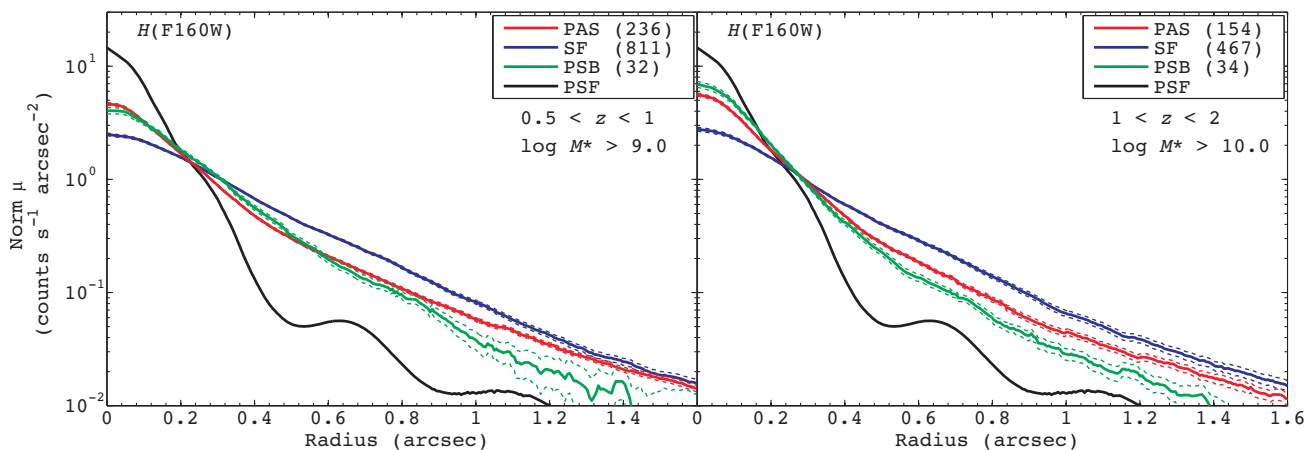
Figure 4. Median-stacked H_{F160W} light profiles \tilde{\mu}(r) for different galaxy populations and at different epochs. Left-hand panel: \tilde{\mu}(r) profiles for passive (PAS; red line), star-forming (SF; blue line), and PSB galaxies (green line) at 0.5 < z < 1 . Right-hand panel: analogous \tilde{\mu}(r) profiles at 1 < z < 2 . The errors in the \tilde{\mu}(r) profiles (dashed lines) are 1\sigma confidence limits, which are determined from the mean of the standard errors from 100 simulated stacks generated via a bootstrap method. The respective sample sizes used to generate the \tilde{\mu}(r) profiles are shown in the legend. The HST H_{F160W} PSF profile (black line) is also shown for reference. Virtually identical \tilde{\mu}(r) profiles are also obtained from the J_{F125W} imaging.
