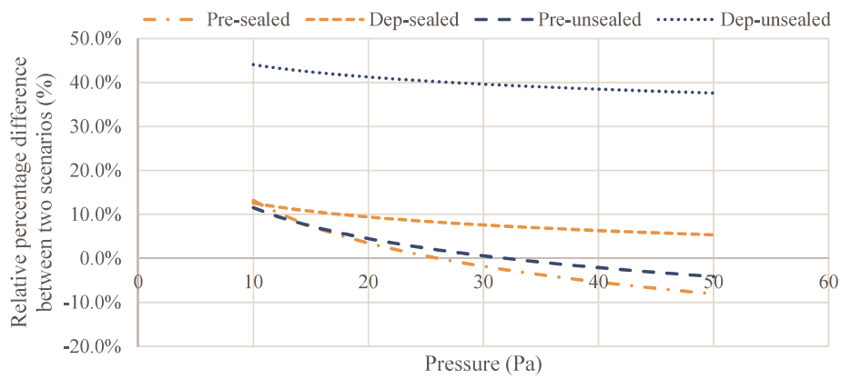
Figure 9 Relative percentage difference (RPD) of blower door test results against the pulse results in sealed and unsealed condition
