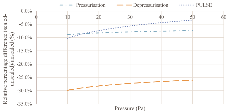
Figure 10 Impact of the sealed testing condition on the pulse and blower door test results
