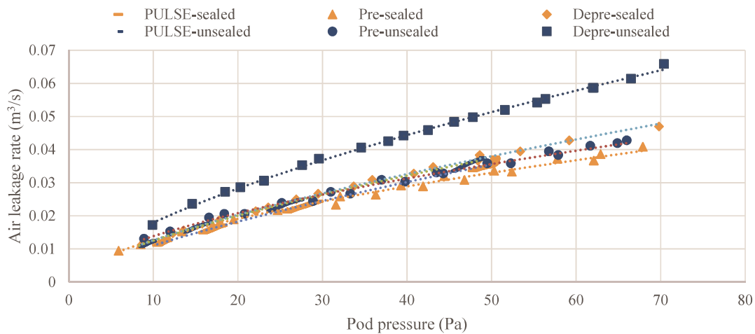
Figure 8 Pressure-leakage curves measured by both methods with and without sealing in pod 1
