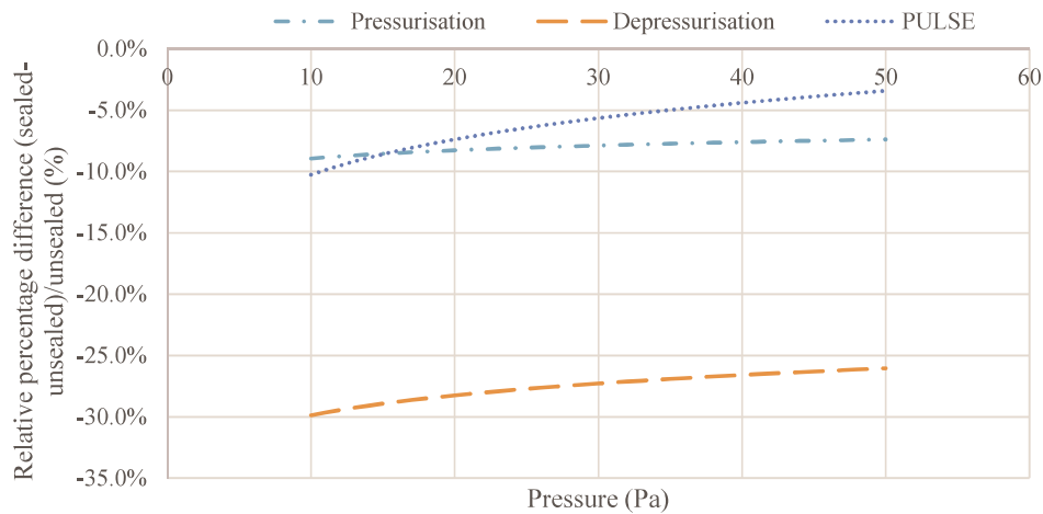
Figure 10. By sealing the gaps, the pulse test measured leakage rate of the pod envelope is reduced by 10.3% at 10 Pa and down to 3.4% at 50 Pa. For the blower door test with the pressure increasing from 10 Pa to 50 Pa, the reduction in the measured leakage changed by 29.9% to 26% in the depressurisation test, and by 8.9% to 7.4% in the pressurisation test. Hence, when applying the sealing the measured leakage of the pod envelope shows the greatest impact on the blower door depressurisation test, followed by the pressurisation test and with the smallest impact on the pulse test. This would seem intuitive given that the blower door frame is a temporary fixture and liable to some movement when under a sustained pressure differential.
