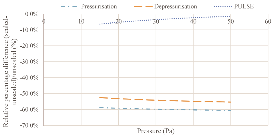
Figure 13 Impact of sealed condition on the pulse and blower door test results
