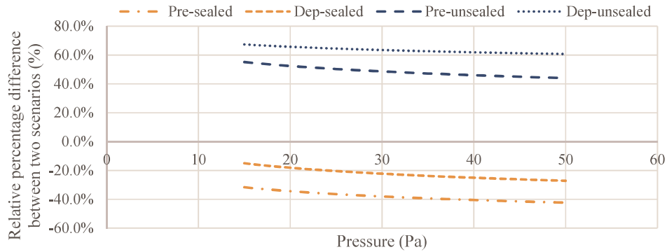
Figure 12 Relative percentage difference (RPD) of blower door test results against the pulse results in sealed and unsealed condition
