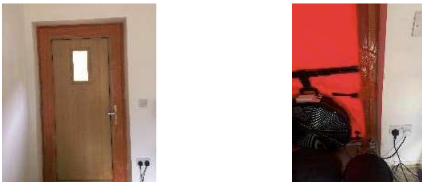
Figure 7 Sealing preparations (light red edging tape) in pulse (left) and blower door (right) test
