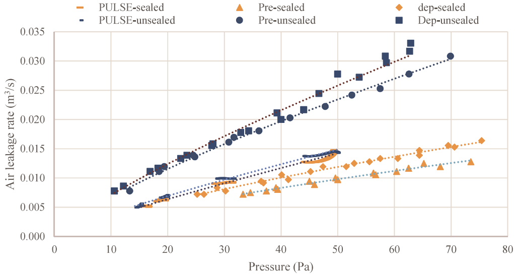
Figure 11 Pressure-leakage curves measured by both methods with and without sealing of Pod 2
