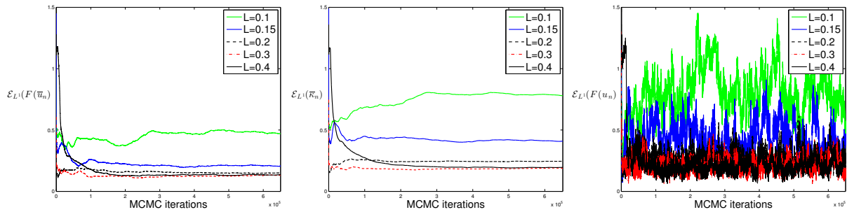
Figure 6: Inverse Potential. L^1(D) relative errors with respect to the truth for different choices of L . Left: \mathcal{E}_{L^1}(F(\bar{u}_n)) . Middle: \mathcal{E}_{L^1}(\bar{\kappa}_n) . Right: \mathcal{E}_{L^1}(F(u_n))
