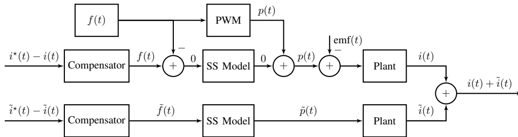
(d) By linearity, the lower branch of (c) can be split into two separate branches.
