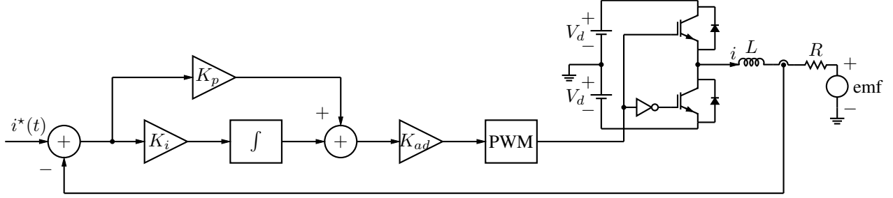
Figure 8: Circuit used for the design example.
