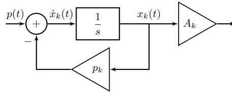
Figure 18: Block diagram representation of each of the terms of the partial fraction expansion of Eq. (5).
