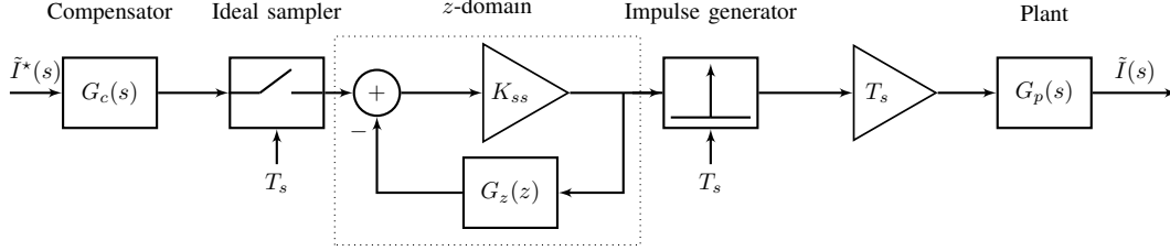
Figure 6: Equivalent block-diagram representation of Fig. 5. Note that the only feedback loop is in the z -domain.
