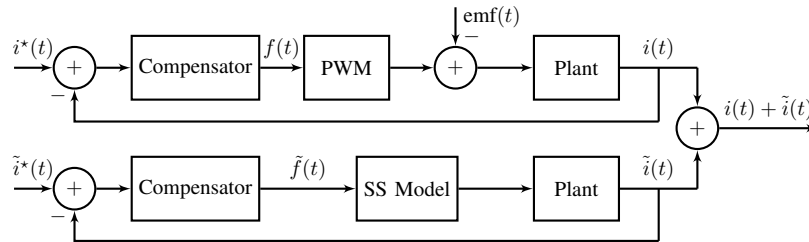
(e) The top branch of (d) is replaced by (a).
