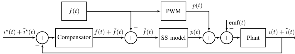
(c) Equivalent representation of the block diagram in (b).
