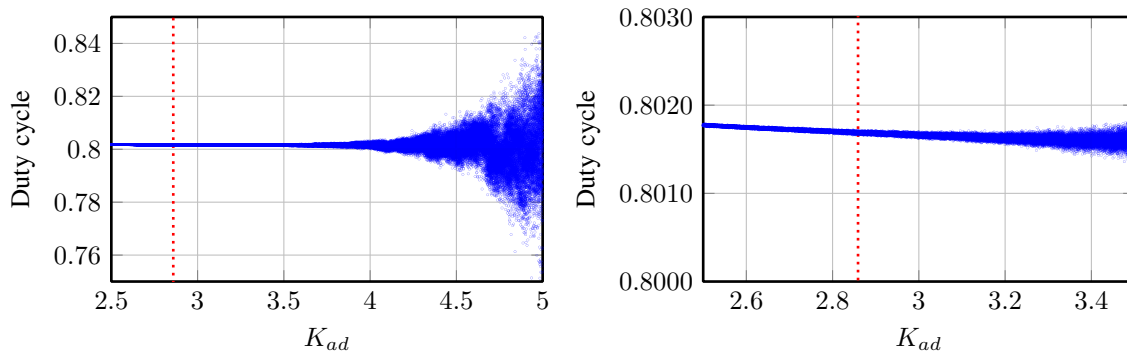
Figure 16: Bifurcation diagram with a sinusoidal reference current. The dotted line indicates the critical loop gain. The figure on the right is a zoomed view near the bifurcation point.
