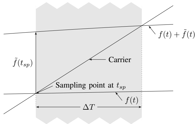
Figure 2: Zoomed view of the perturbed and unperturbed intersection points, leading to a narrow rectangular pulse.
