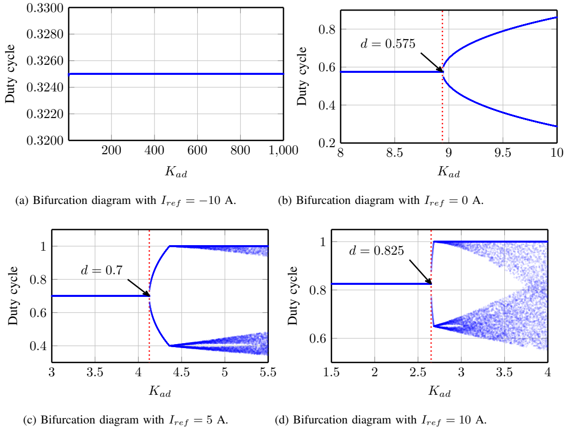
Figure 13: Bifurcation diagrams. The dotted lines show the theoretical value of the critical loop gain.
