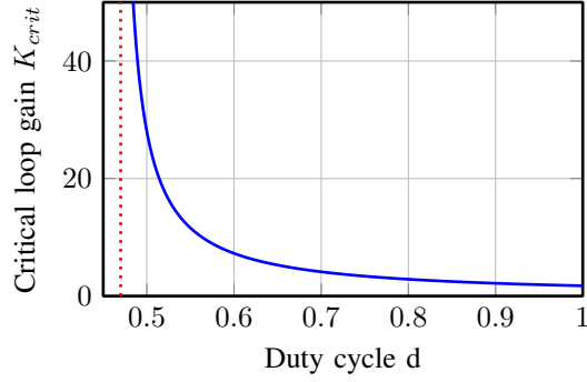
Figure 12: Critical gain K_{crit} as a function of duty cycle. The red asymptote is located at d = 0.47 .
