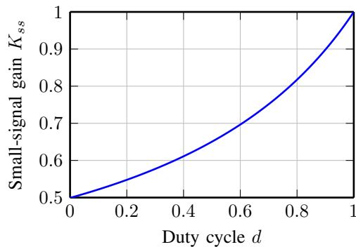
Figure 9: Small-signal gain as a function of duty cycle.
