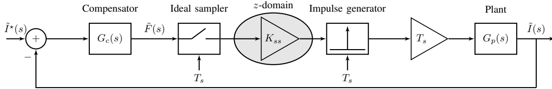
Figure 5: PWM small-signal model embedded in the feedback loop.
