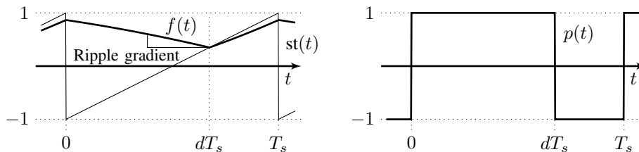
Figure 7: Typical modulator input and output signals in the steady state.
