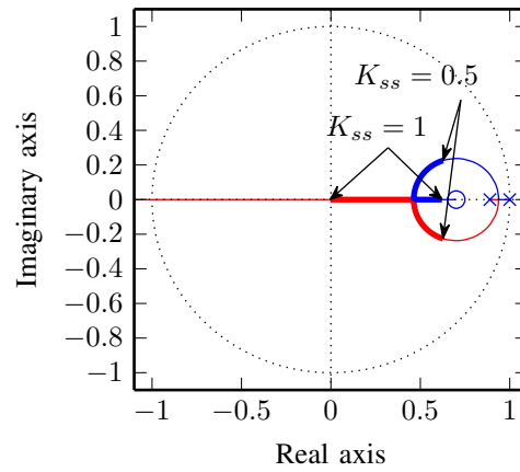
Figure 11: z -domain root locus.
