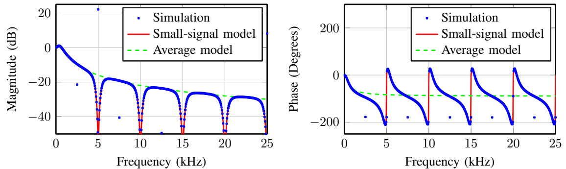
Figure 15: Small-signal closed-loop frequency response. The magnitude response is shown on the left and the phase response on the right.
