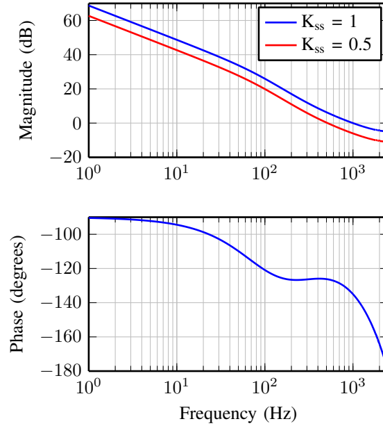
Figure 10: Open-loop z -domain bode plot.
