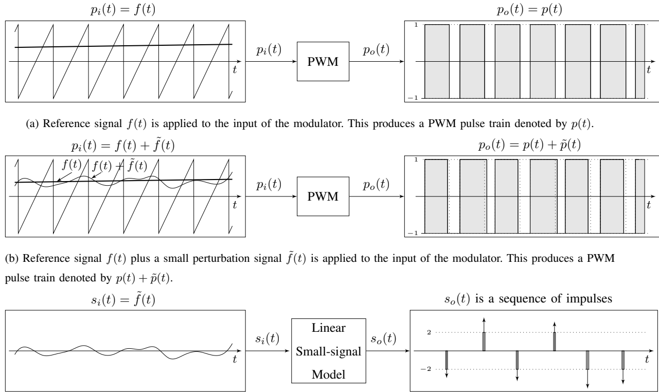
(a) Reference signal f(t) is applied to the input of the modulator. This produces a PWM pulse train denoted by p(t) . (b) Reference signal f(t) plus a small perturbation signal \tilde{f}(t) is applied to the input of the modulator. This produces a PWM pulse train denoted by p(t) + \tilde{p}(t) . (c) The sequence \tilde{p}(t) of narrow rectangular pulses is the difference between the PWM pulse trains in (a) and (b). This sequence of narrow rectangular pulses is modelled as a sequence of impulses. The strength of each impulse is equal to the area of the narrow rectangular pulse it represents.
