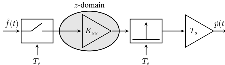
Figure 3: Small-signal model of the single-edge pulse-width modulator.
