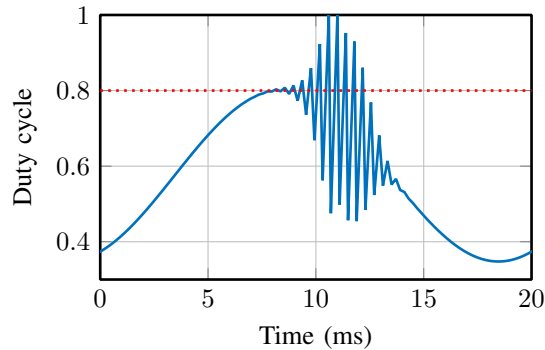
Figure 17: Duty cycle d over one 20 ms cycle with a sinusoidal reference and K_{ad} = 4.25 . The dotted red line shows the theoretical value of d at which instability is expected.
