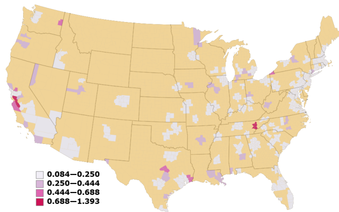
(c) \sigma^2
