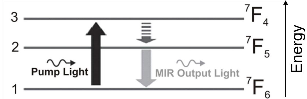
Figure 2. Energy level diagram for a terbium ion doped into selenide chalcogenide glass
