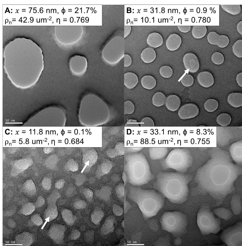
Figure 2. NPN membranes manufactured with different nanomorphologies. (A–D) TEM images (63 kx, 0^\circ ) of four different varieties of NPN. The sizes and shapes of the pores can range from largely open (A,D) to pitted and under-etched (B,C). White arrows indicate open nanopores in low-porosity films. Parameters derived from histograms of counted pores (Supplemental Section S1) show the wide variety of membrane porosities and pore diameters. x = Average Pore Diameter, \Phi = Porosity, \rho_n = Pore Density, \eta = Circularity.
