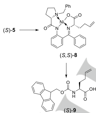
Scheme 3. The synthetic route to Fmoc-homoallylglycine-OH.
